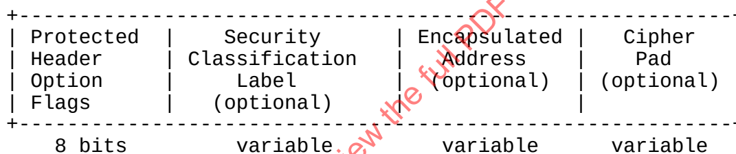
Figure 3-3: SCPS-SP Protected Header
