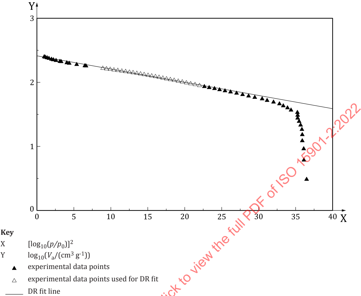
Figure 6 — Dubinin-Radushkevitch (DR) plot of an adsorption isotherm of N 2 at 77 K on activated carbon
