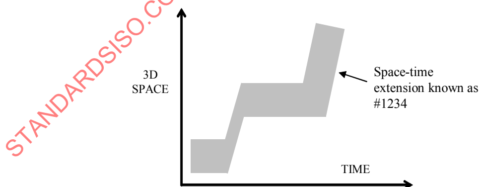
Figure 7 — Possible individual as a space-time extension
