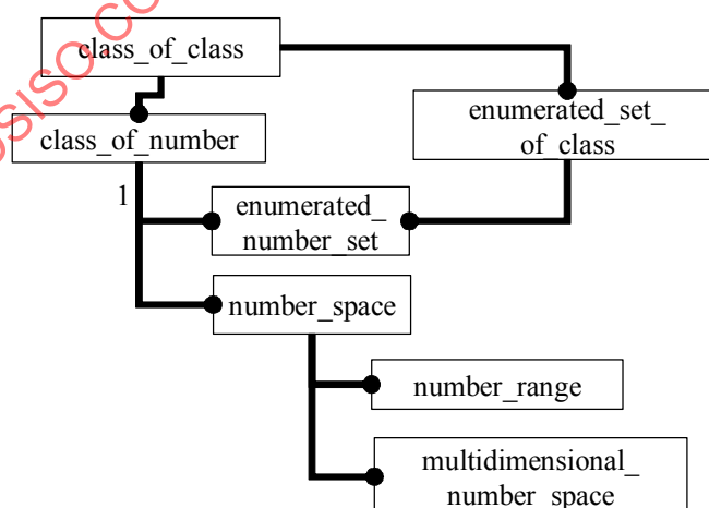
Figure 157 — Class of number
