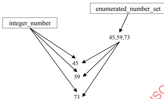
Figure 158 — Enumerated number set
