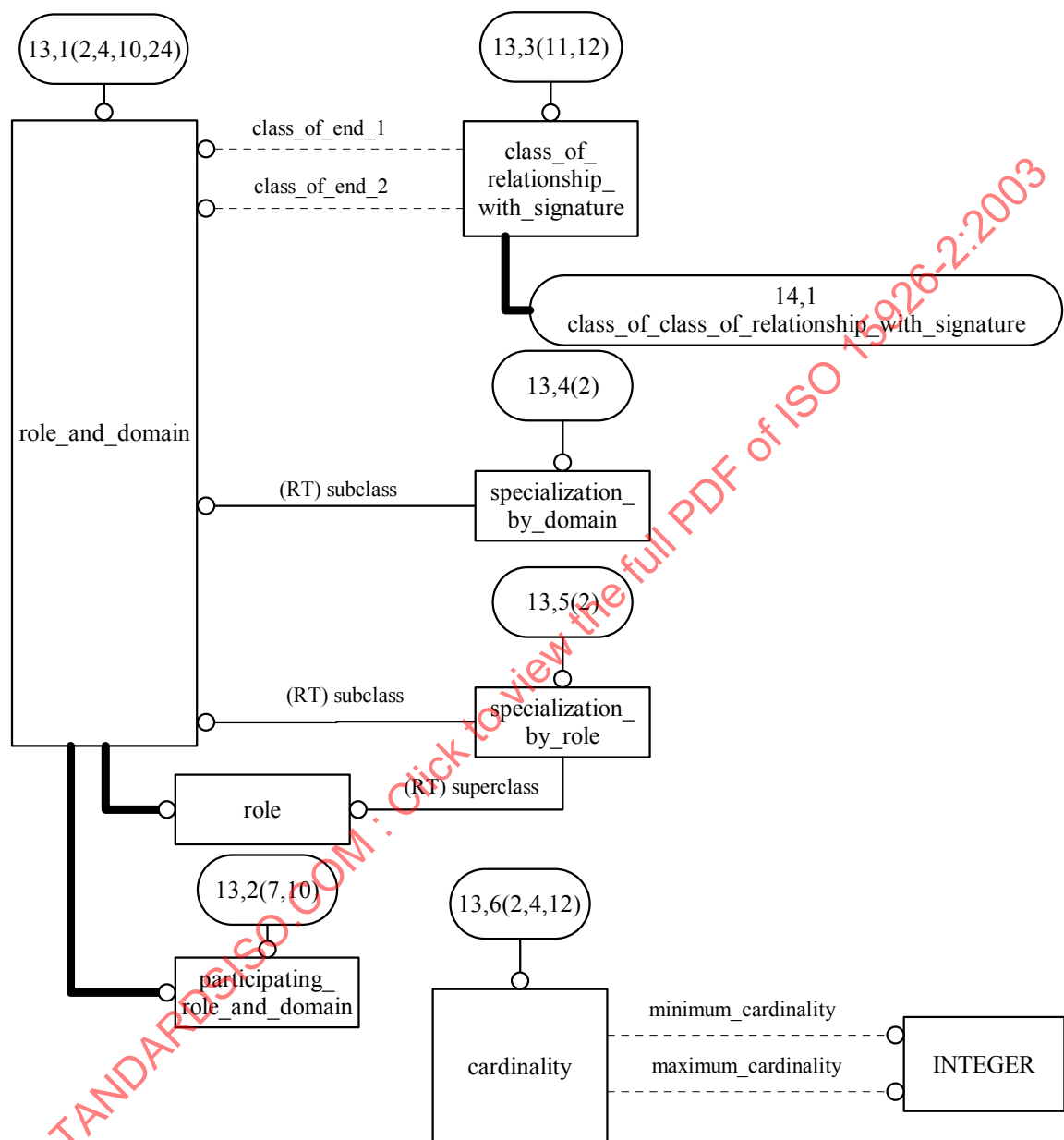
Figure 189 — lifecycle_integration_schema EXPRESS-G diagram 13 of 29
