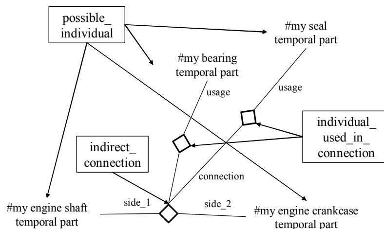
Figure 19 — Shaft crankcase indirect connection
