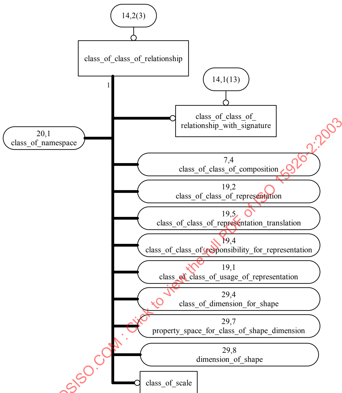
Figure 190 — lifecycle_integration_schema EXPRESS-G diagram 14 of 29
