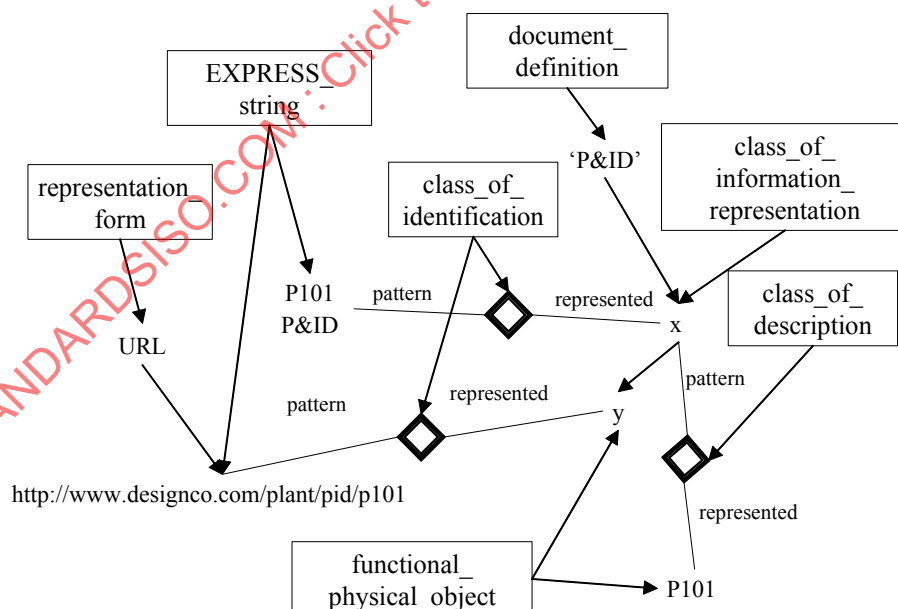
Figure 104 — P101 P&amp;ID URL
