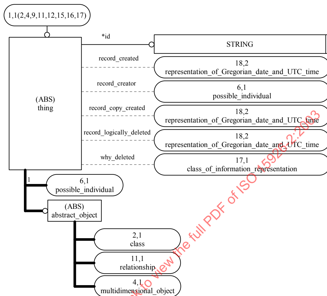
Figure 177 — lifecycle_integration_schema EXPRESS-G diagram 1 of 29
