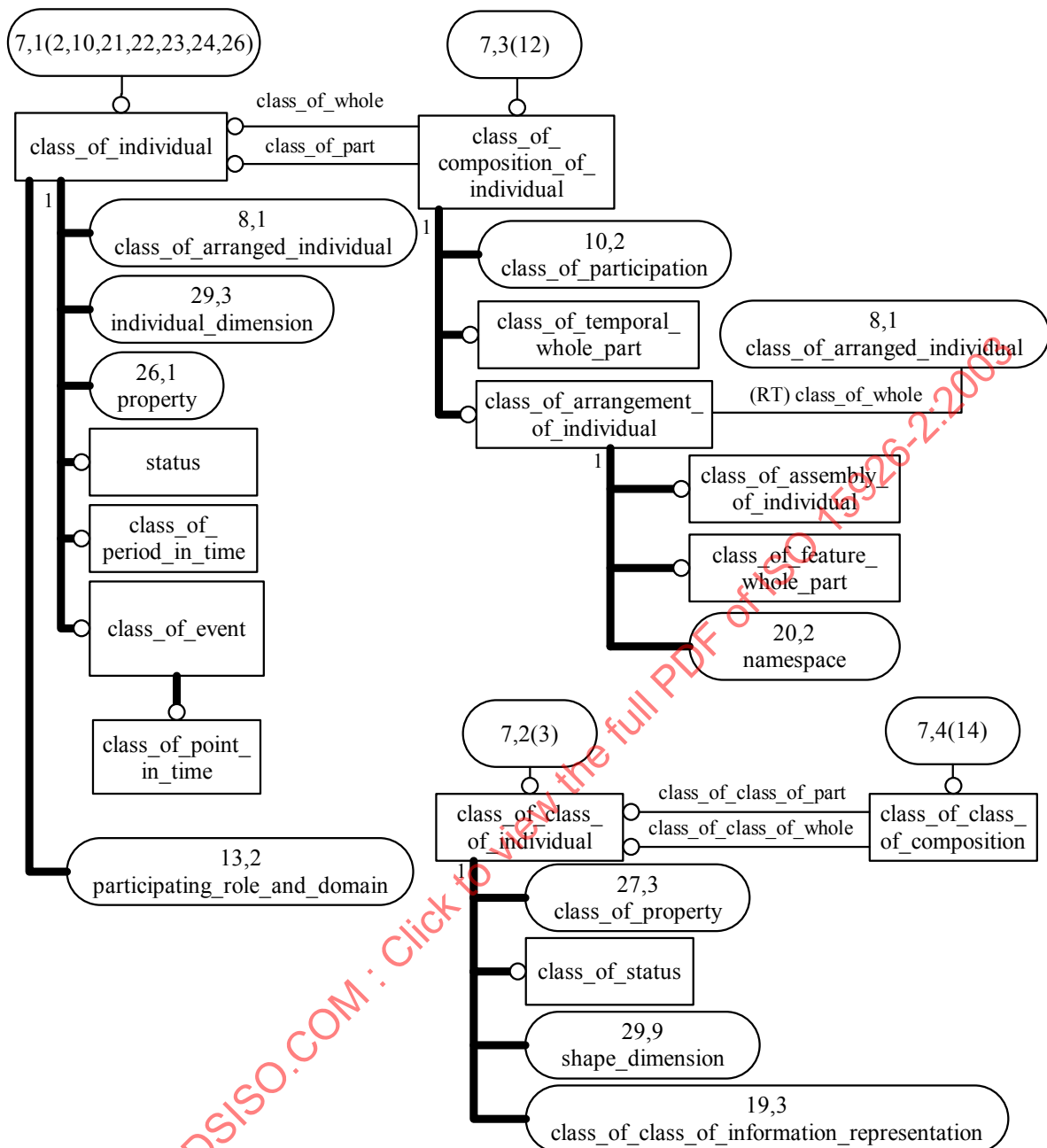
Figure 183 — lifecycle_integration_schema EXPRESS-G diagram 7 of 29
