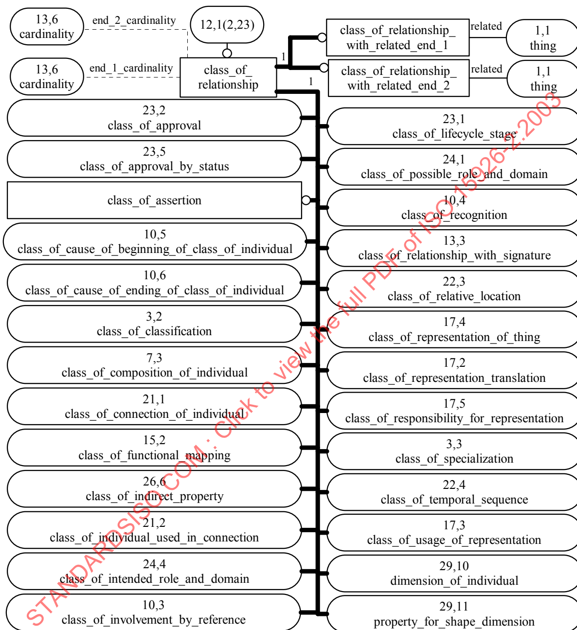
Figure 188 — lifecycle_integration_schema EXPRESS-G diagram 12 of 29
