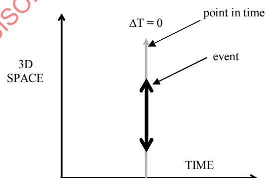
Figure 39 — Point in time extensions
