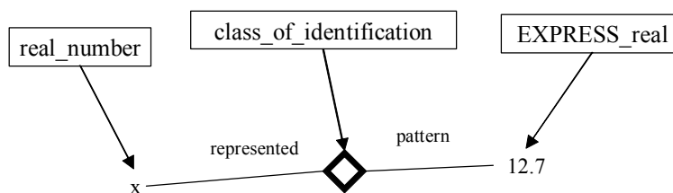
Figure 155 — Representation of real number
