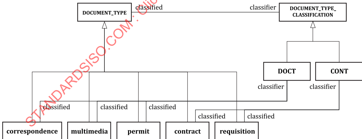
Figure 1 — A UML class diagram related to classifications
