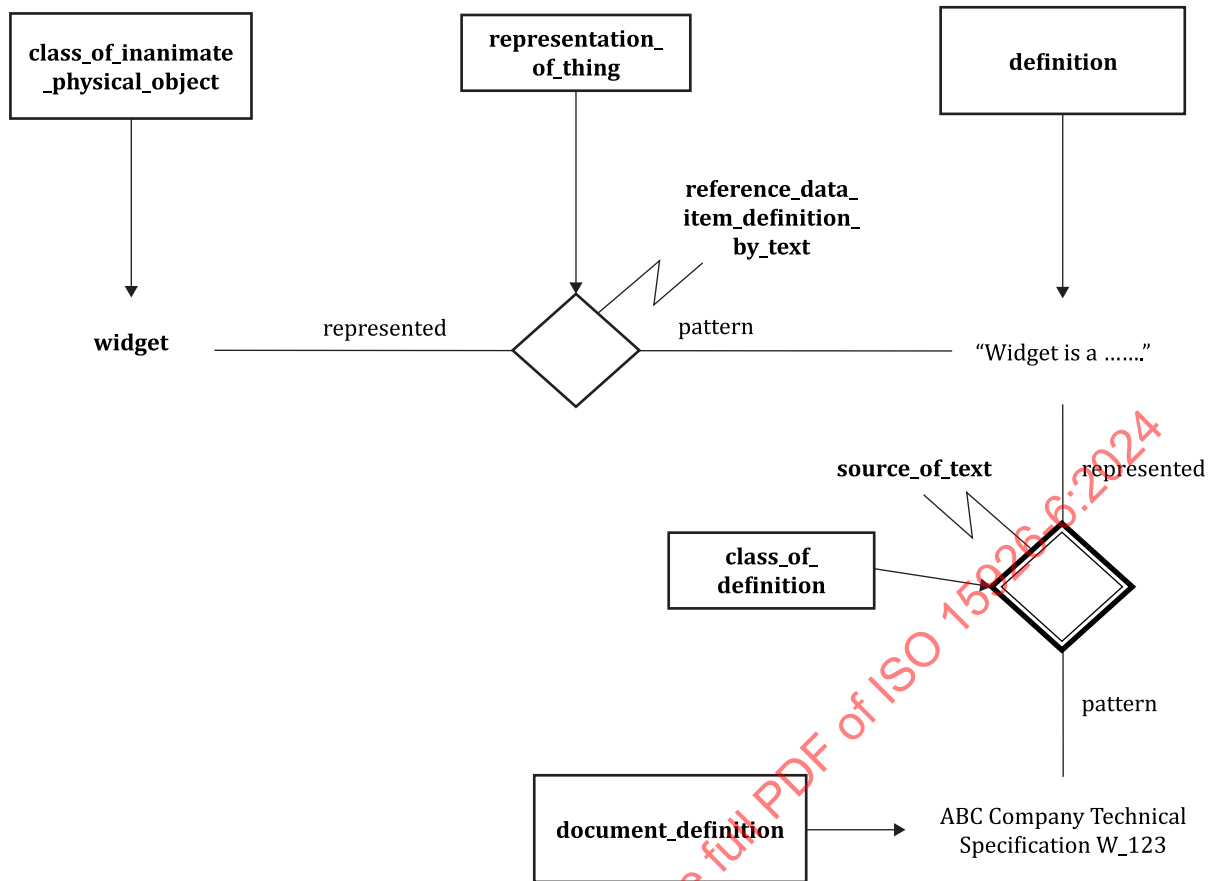
Figure 2 — Source of text as an instantiation of entity types defined in ISO 15926-2
