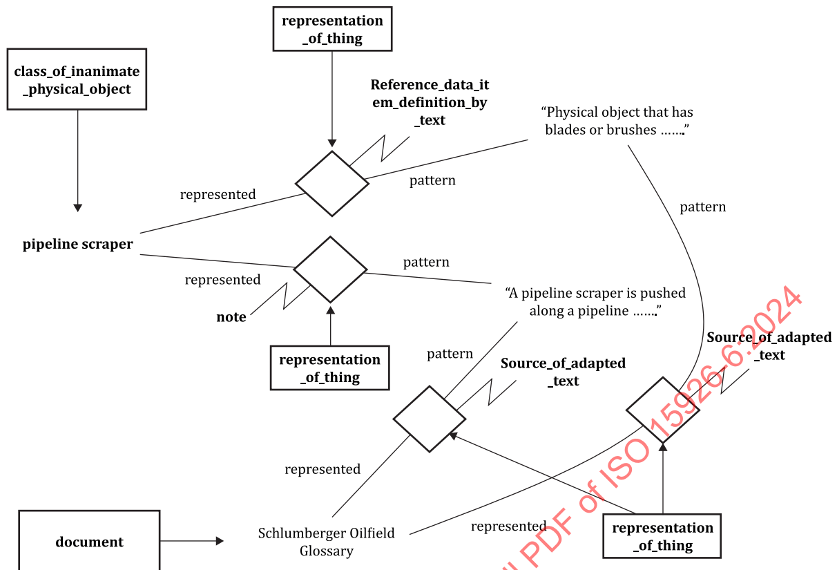
Figure 3 — Source of adapted text as an instantiation of entity types defined in ISO 15926-2
