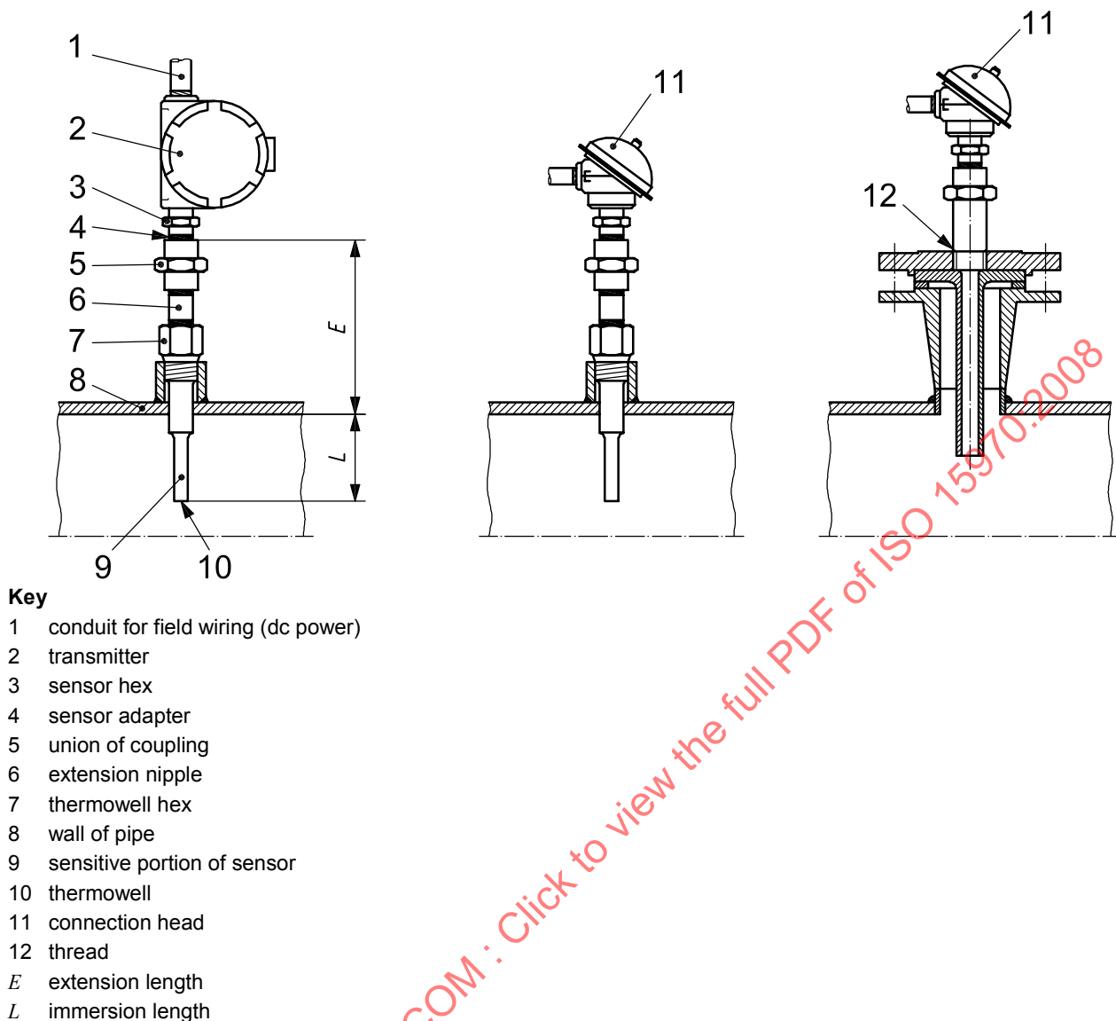
Figure 13 — RTD installation
