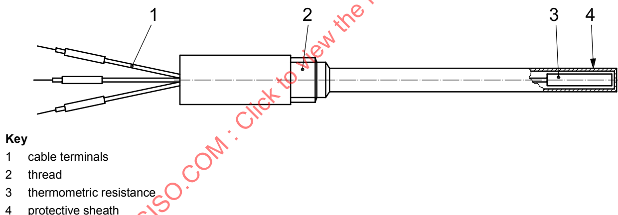
Figure 12 — Typical construction of an RTD
