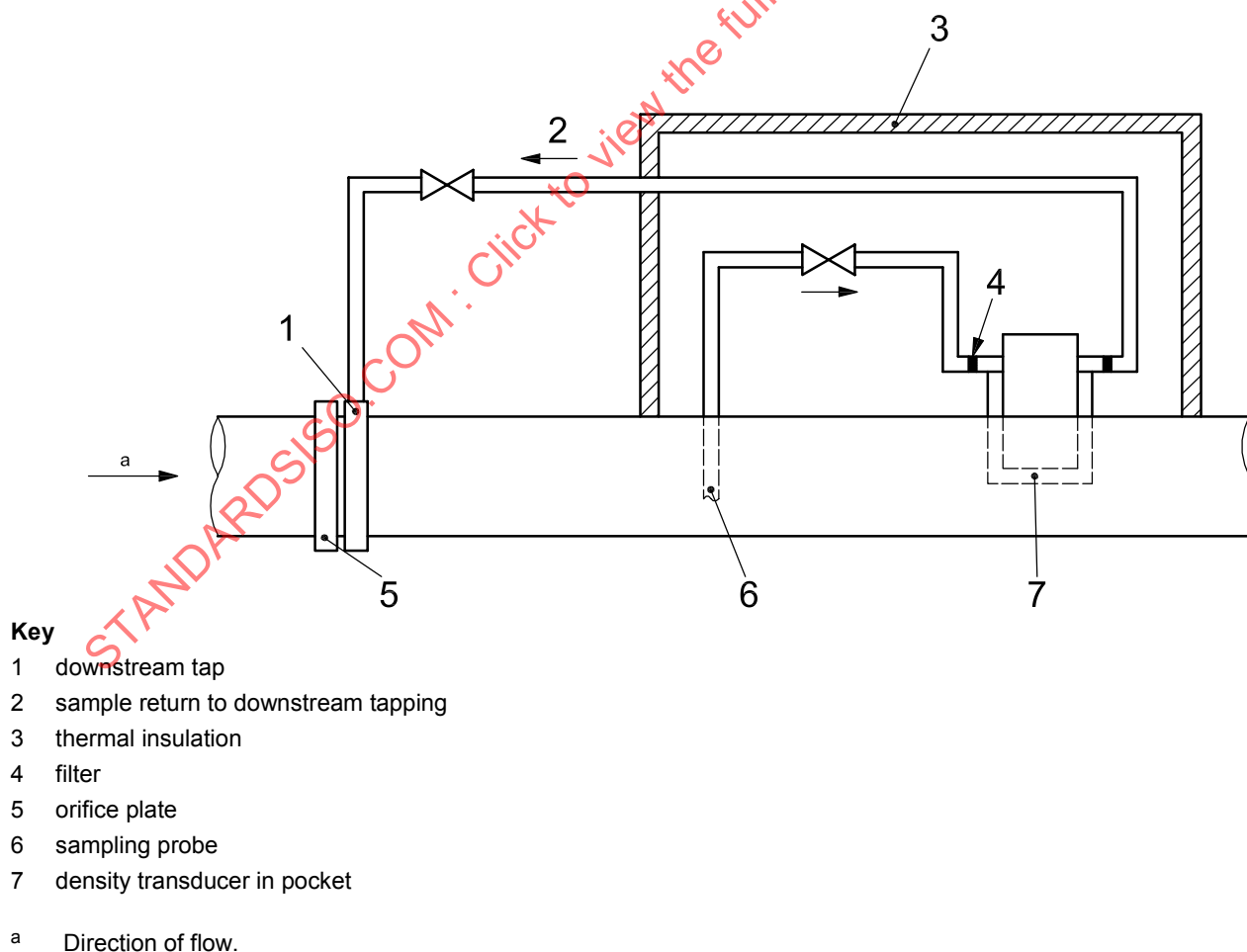
Figure 5 — Installation of a gas-density meter on an orifice plate system for the pressure-recovery method
