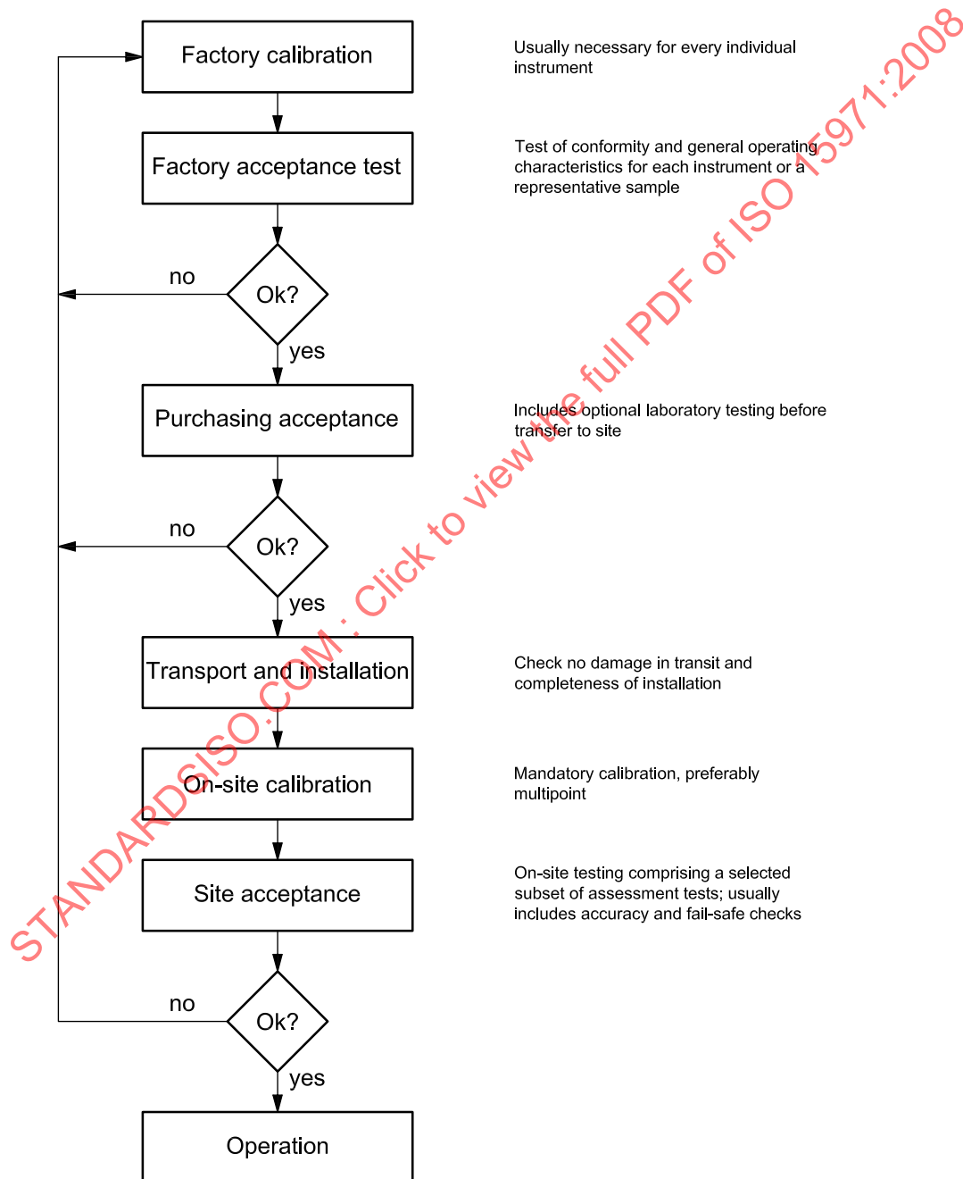
Figure 3 — Factory and site acceptance testing
