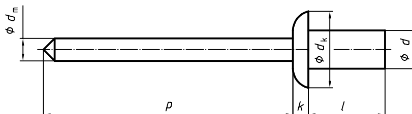
Figure 1 — Rivet dimensions
