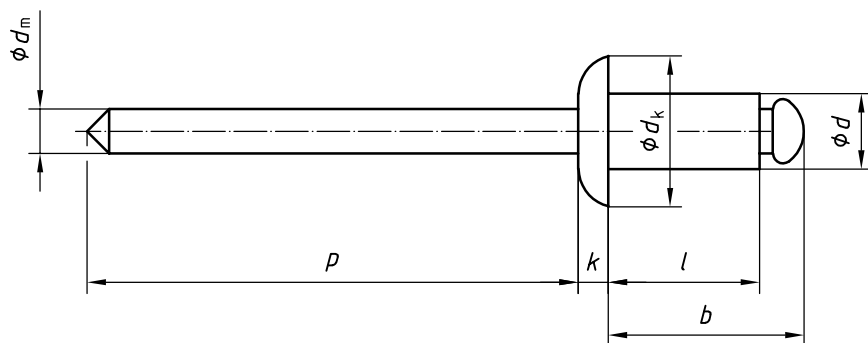
Figure 1 — Rivet dimensions
