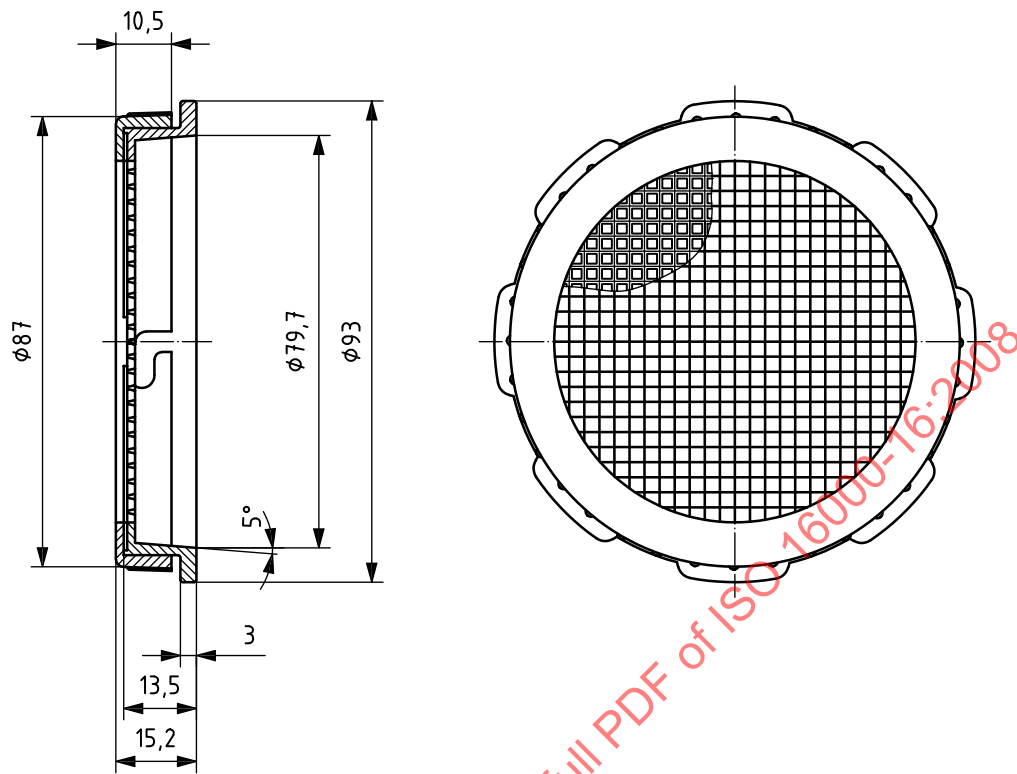
Figure B.2 — Disposable filter holder
