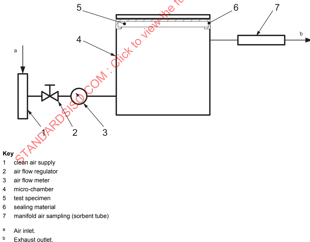
Figure 1 — Schematic diagram of a type of micro-chamber apparatus as used in step 1 of the test
