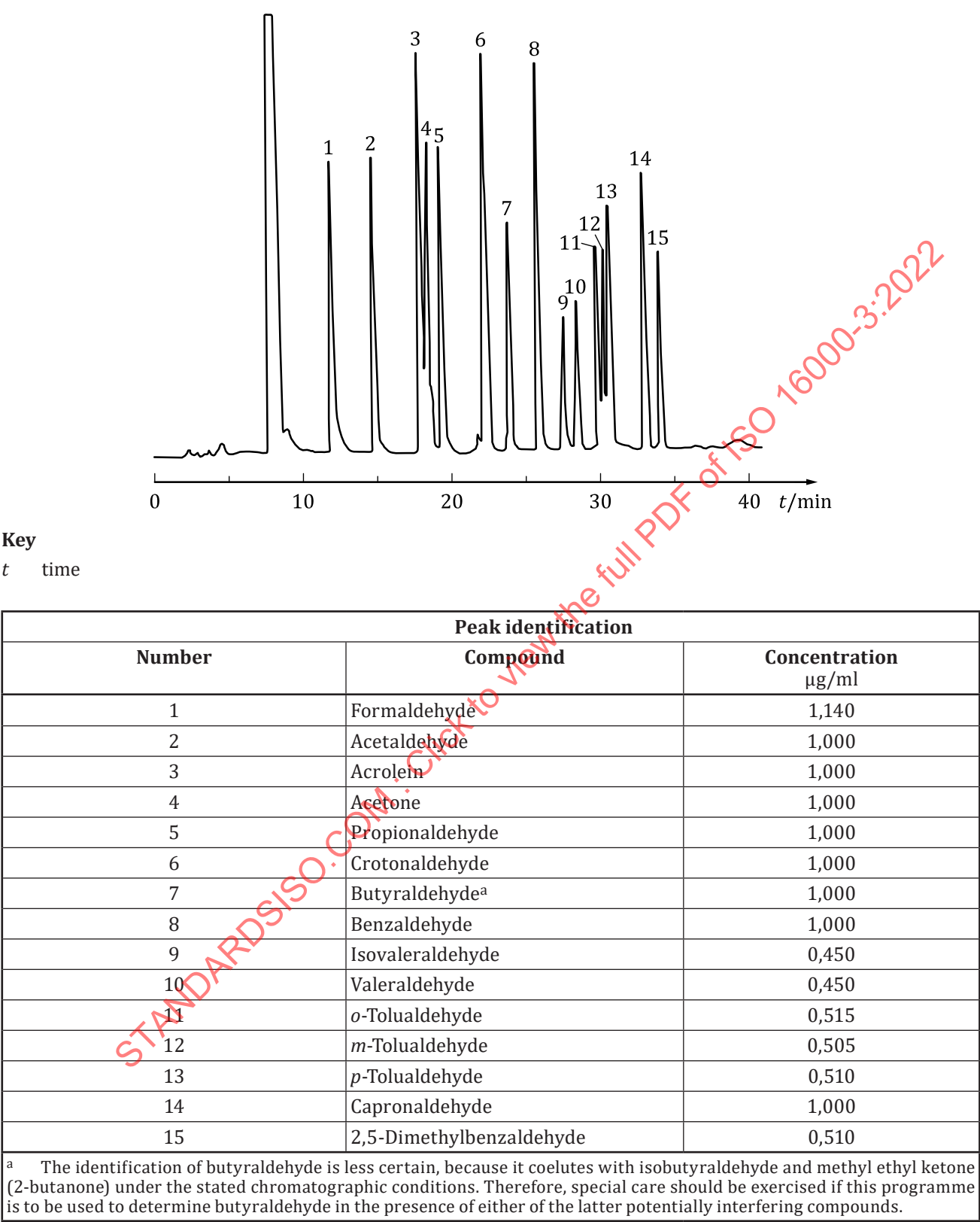
Figure 7 — Example of chromatographic separation of DNPH hydrazones of 15 carbonyl standards
