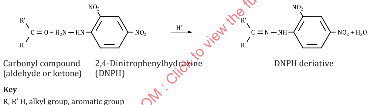
Figure 1 — Reaction of carbonyl compounds to form 2,4-dinitrophenylhydrazones
