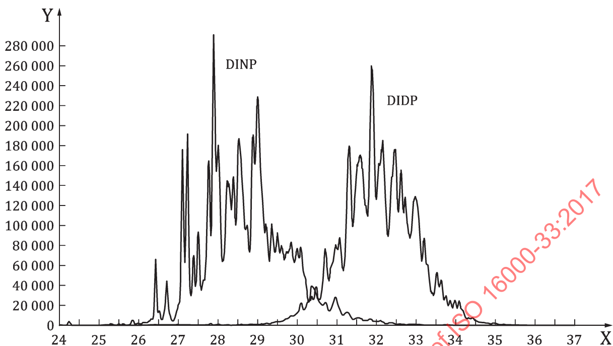
a) Mass trace m/z = 149
