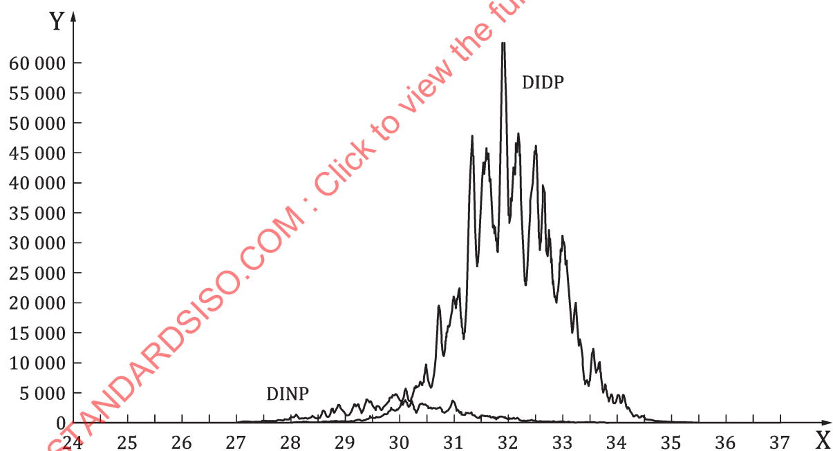
b) Mass trace m/z = 307
