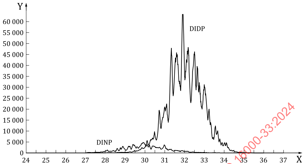
b) Superimposed GC-MS chromatogram of a DiDP standard
