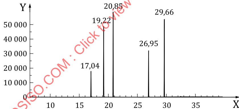
b) Chromatogram of a calibration standard of 1 mg/l b
