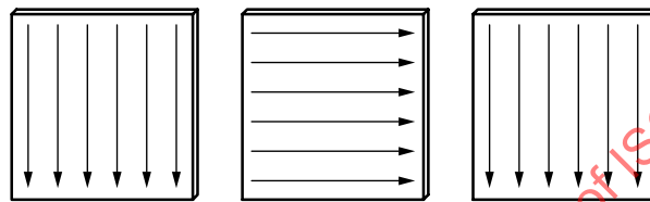
Figure C.2 — Sampling of solvent wipe samples
