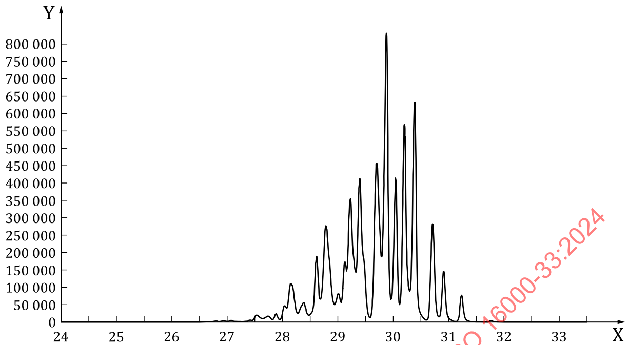
a) GC-MS chromatogram ( m/z = 149 ) for DiNP standard producer A
