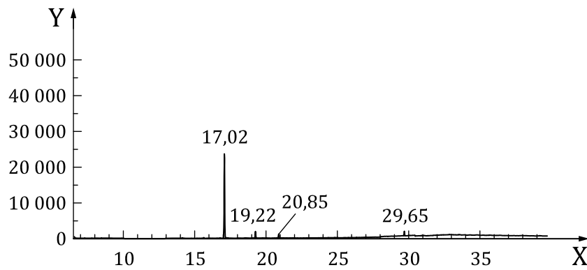
a) Chromatogram of a laboratory blank value from a Florisil® tube spiked with the IS and the concentrate a
