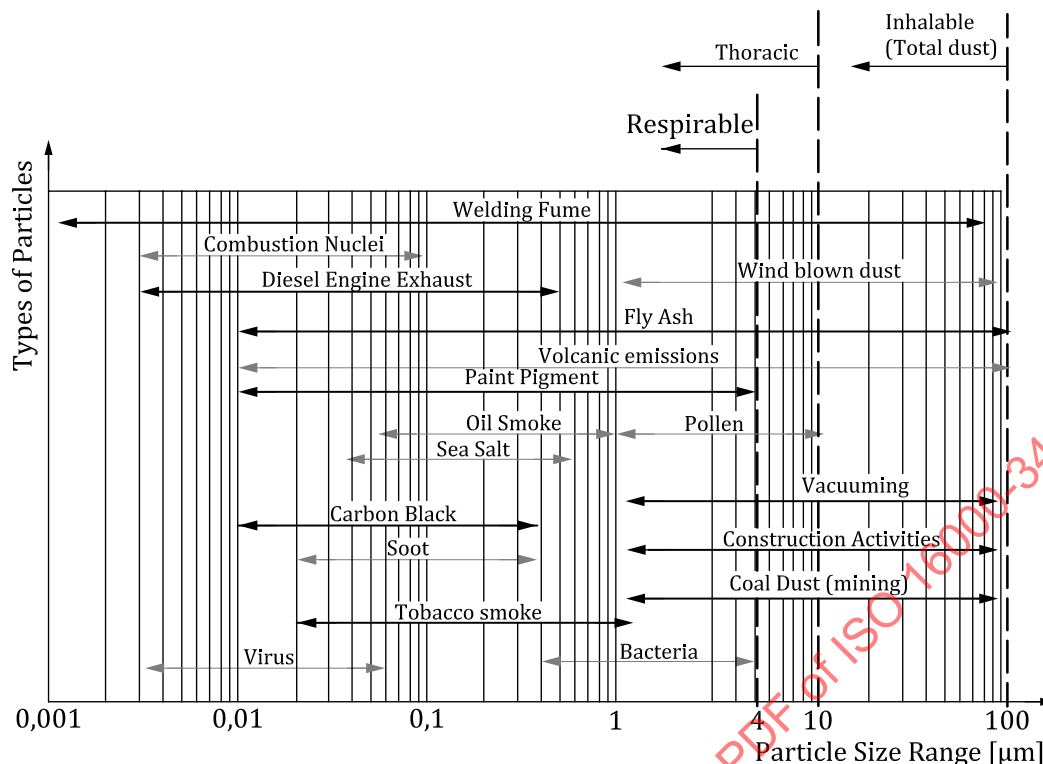
Figure 2 — Typical sources of airborne particles and size ranges
