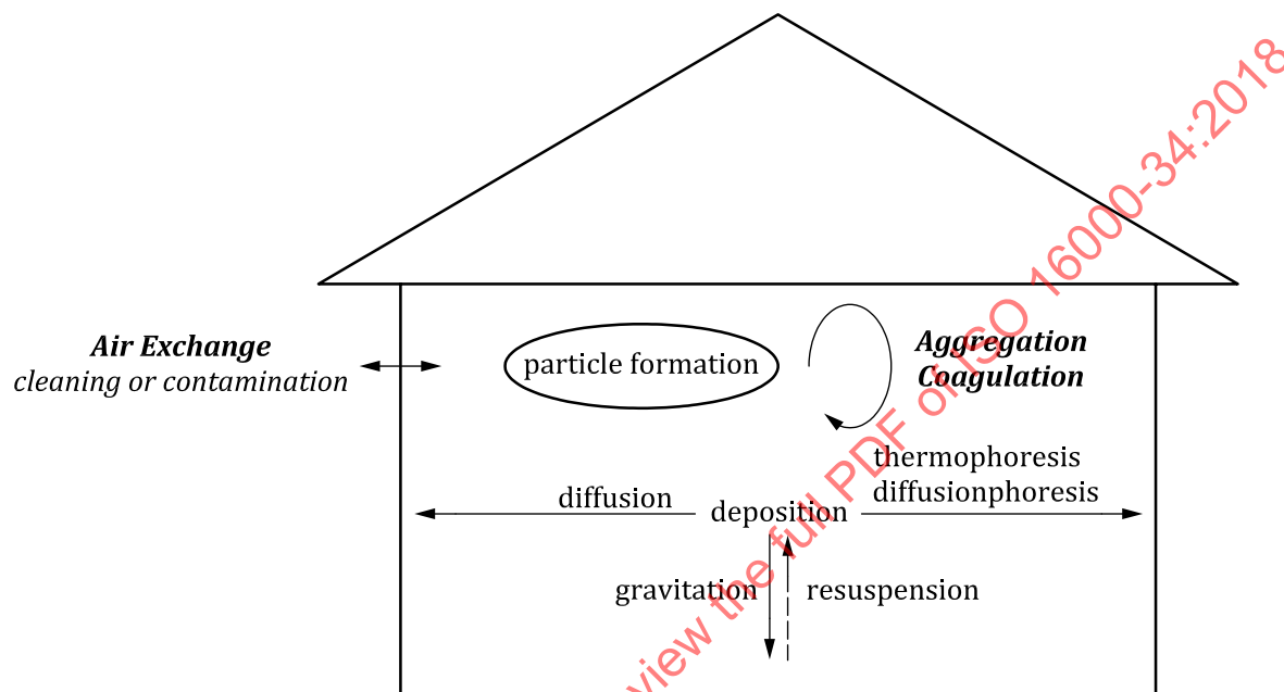
Figure 1 — Particle formation and particle dynamics indoors
