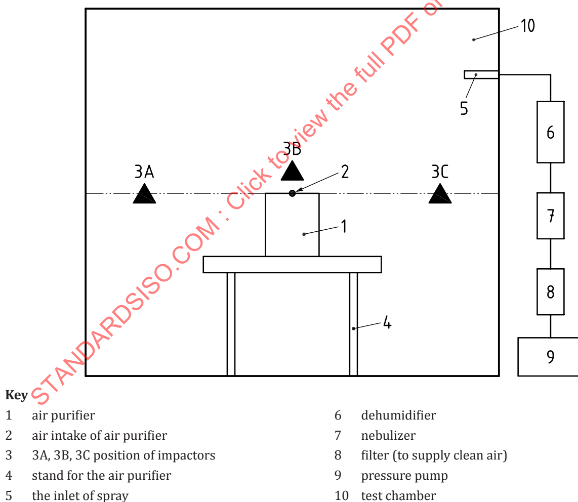
Figure 1 — Schematic diagram of test system using a test chamber
