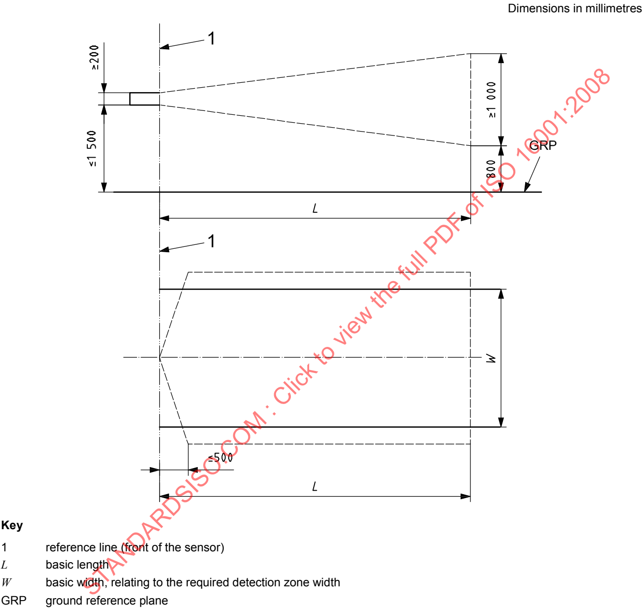
Figure D.1 — Detection zone shape
