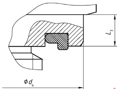
c) Profile seal
