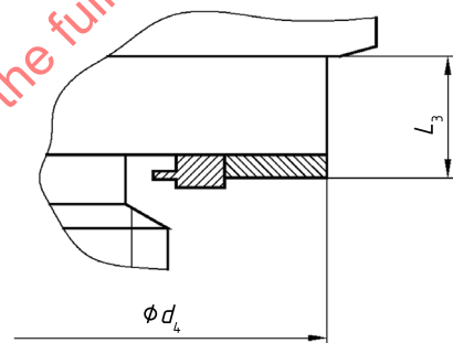
d) Composite seal
