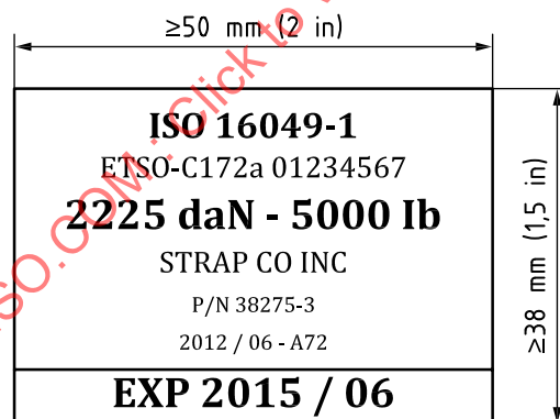
Figure 4 — Typical marking label
