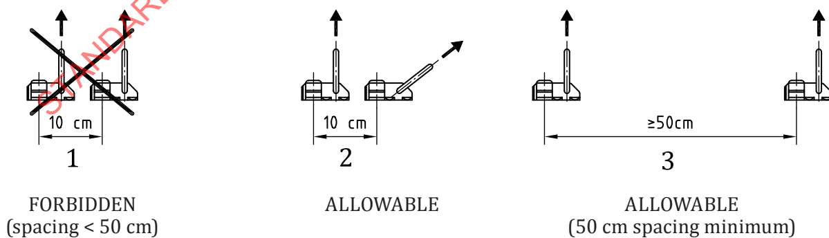
Figure 2 — Minimum distances
