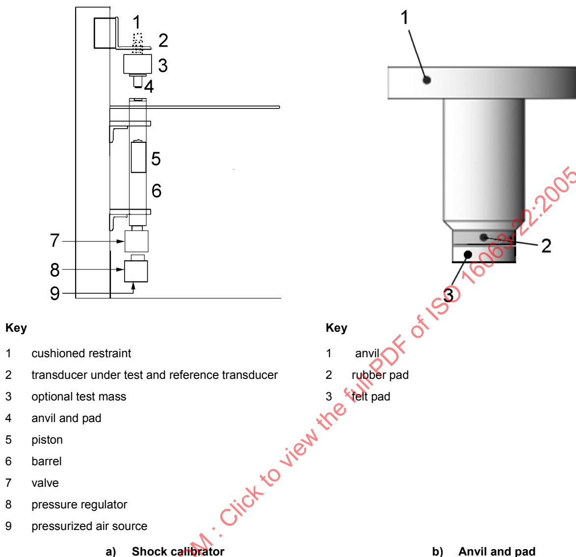
Figure 5 — Schematic diagram for an upwardly moving pneumatically operated piston shock calibrator
