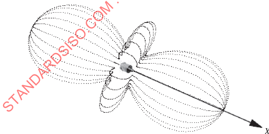
Figure A.3 — Example of an output curve of the transducer in magnetic field in all test planes
