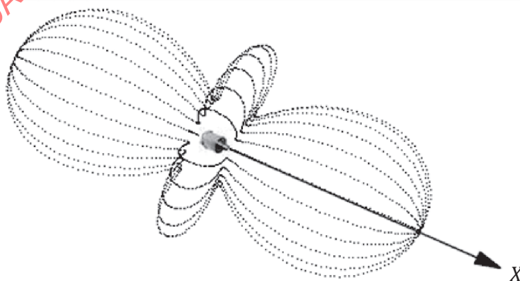
Figure B.4 — Example of an output curve of the transducer in magnetic field in all test planes (all measurements cross the x-axis at 0° and 180°)
