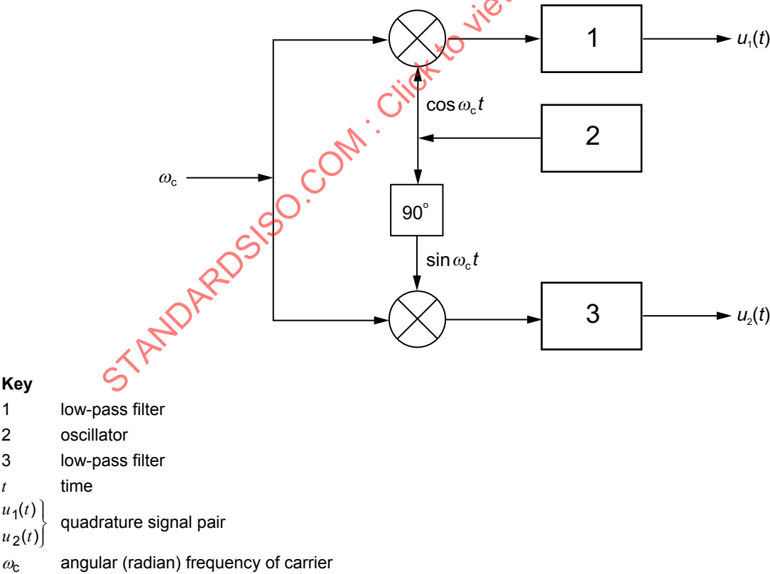
Figure 9 — Conversion of a heterodyne carrier to quadrature format
