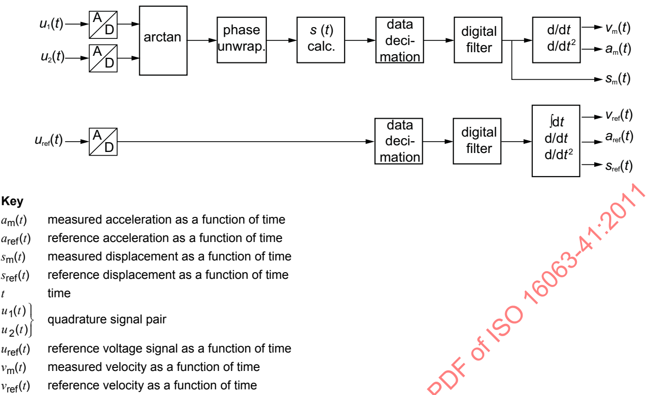
Figure 8 — Example of a numerical signal processing chain of a laser vibrometer standard
