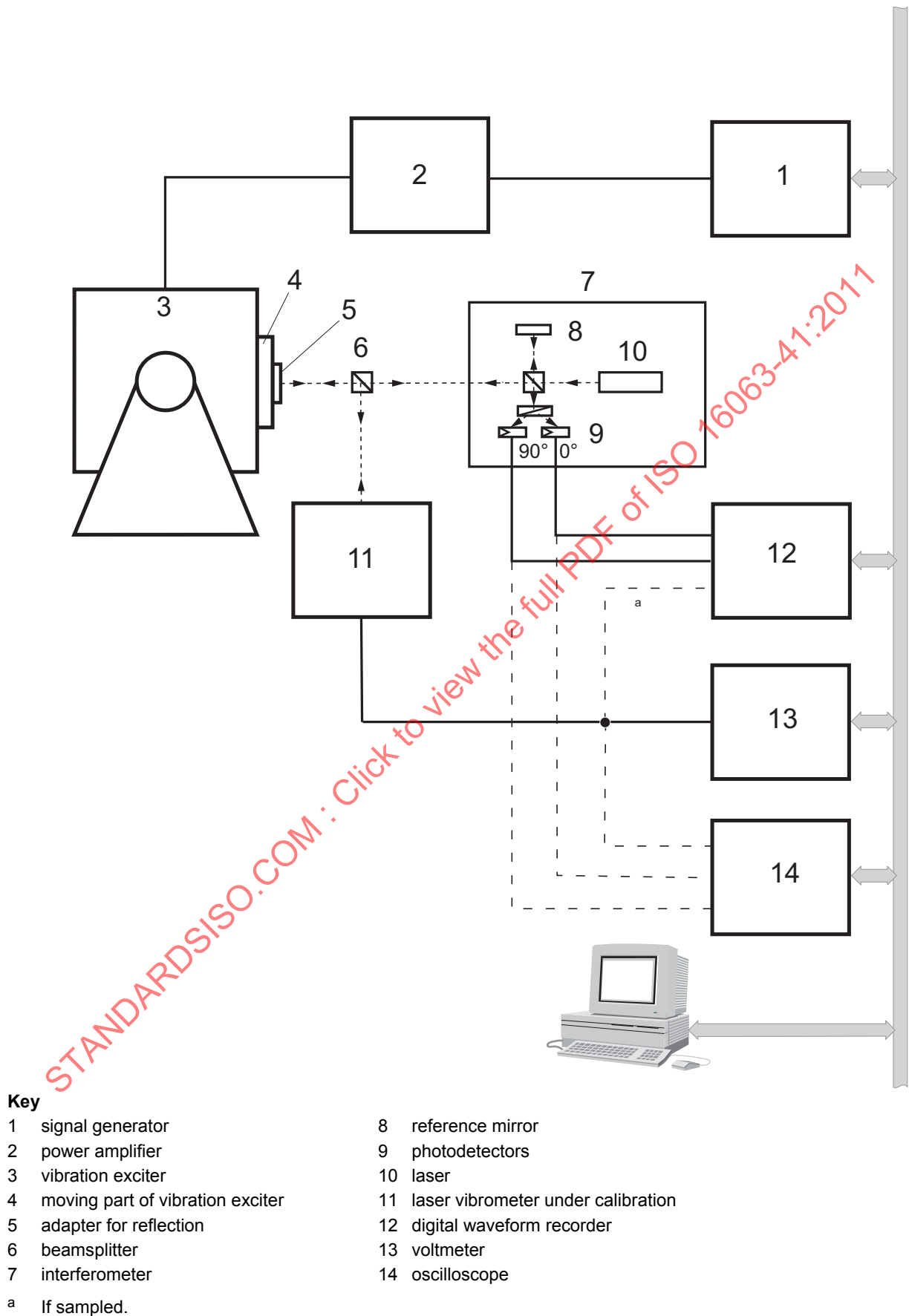
Figure 4 — Example of the measuring system for the sine-approximation method (method 3, homodyne version)
