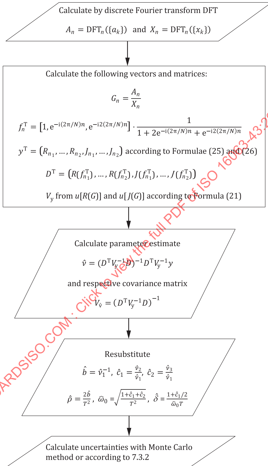
Figure 4 — Flowchart of the process of parameter identification upon shock calibration data in the frequency domain
