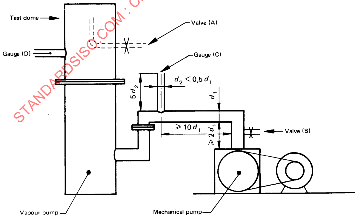
FIGURE 2 — Arrangement of test equipment
