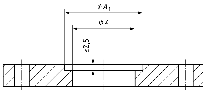
Figure B.2 — Bore for vacuum flanges with recess
