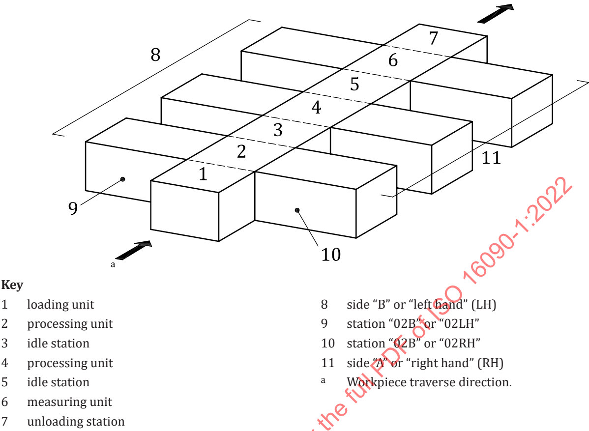
Figure C.11 — Substructure of a transfer machine
