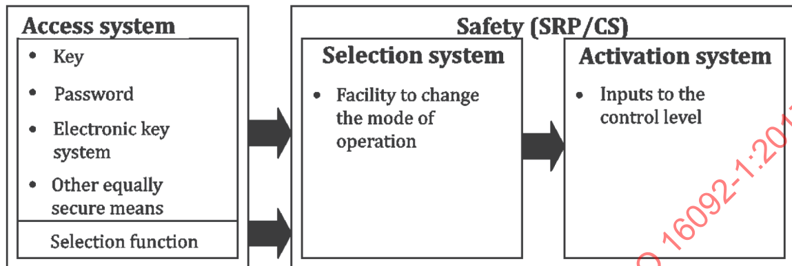
Figure 6 — Border between the access system and the safety system
