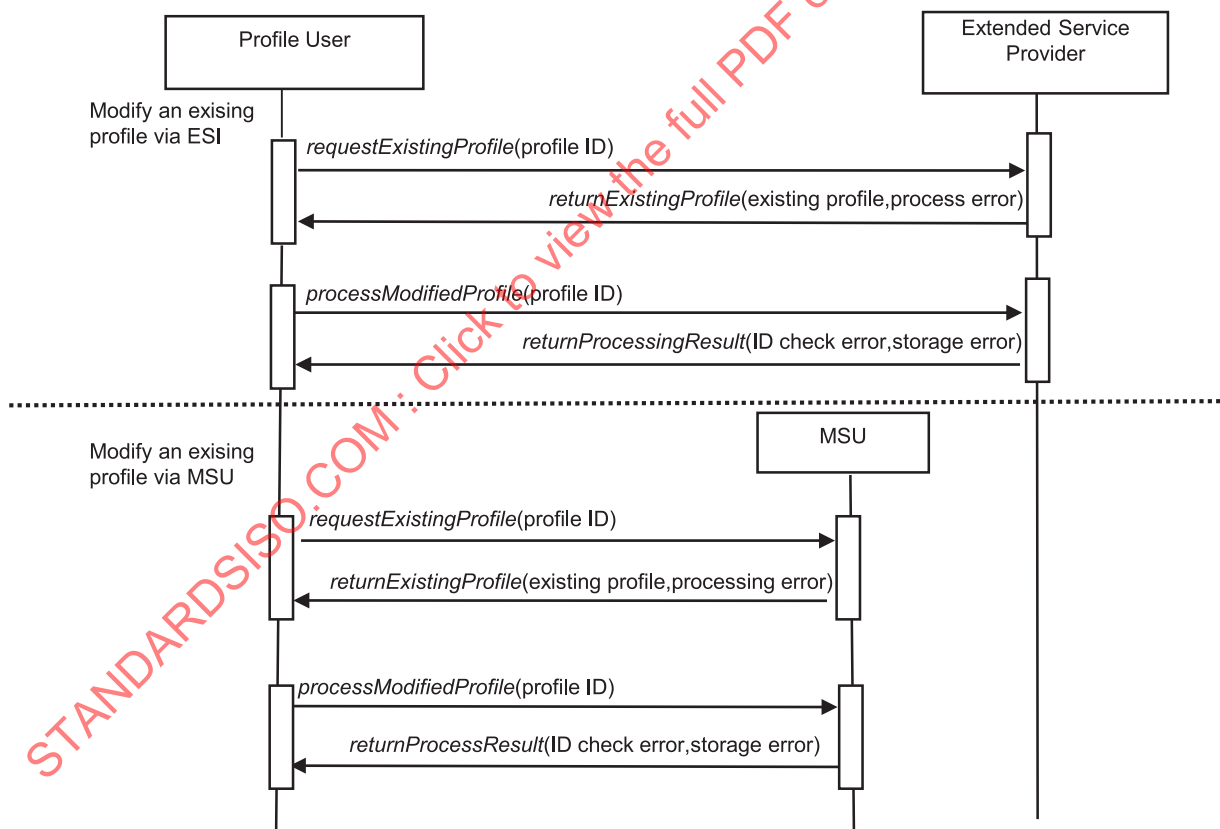
Figure 10 — The modifyProfile service
