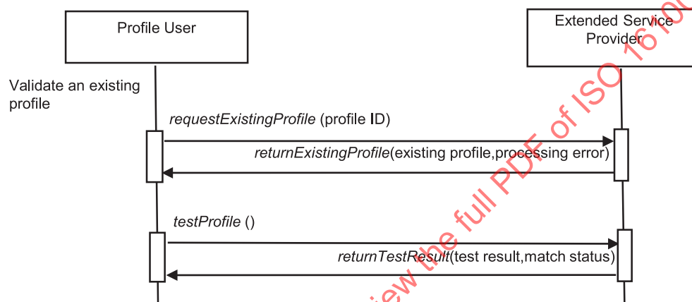
Figure 11 — The validateProfile service
