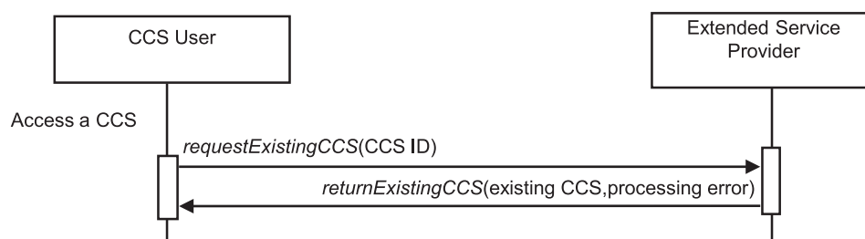
Figure 14 — The accessCCS service
