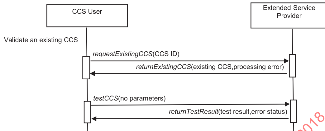
Figure 16 — The validateCCS service
