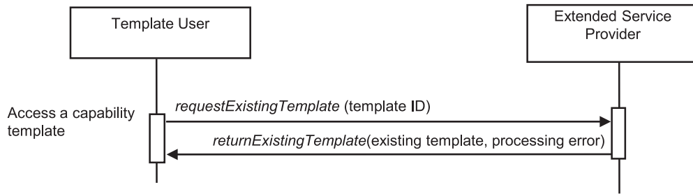
Figure 4 — The accessTemplate service
