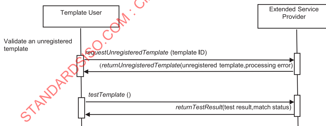
Figure 6 — The validateTemplate service
