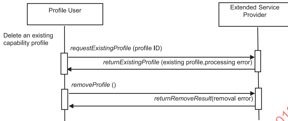
Figure 12 — The deleteProfile service
