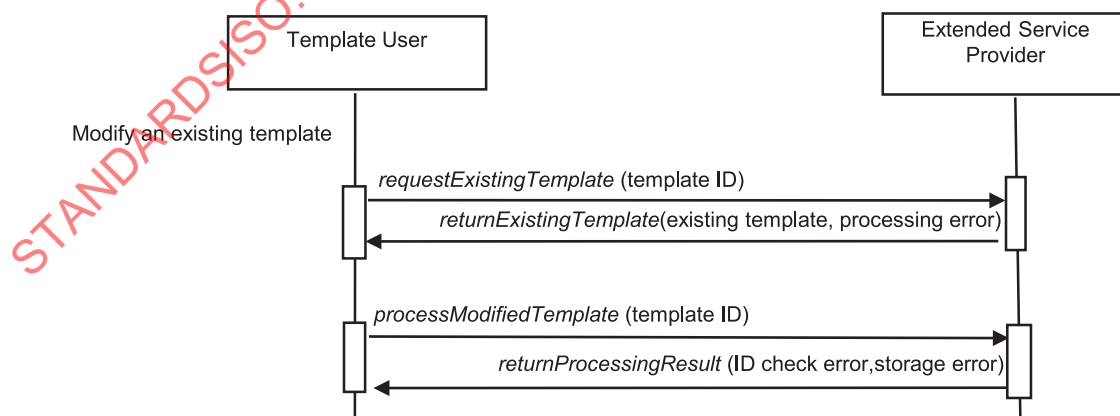
Figure 5 — The modifyTemplate service
