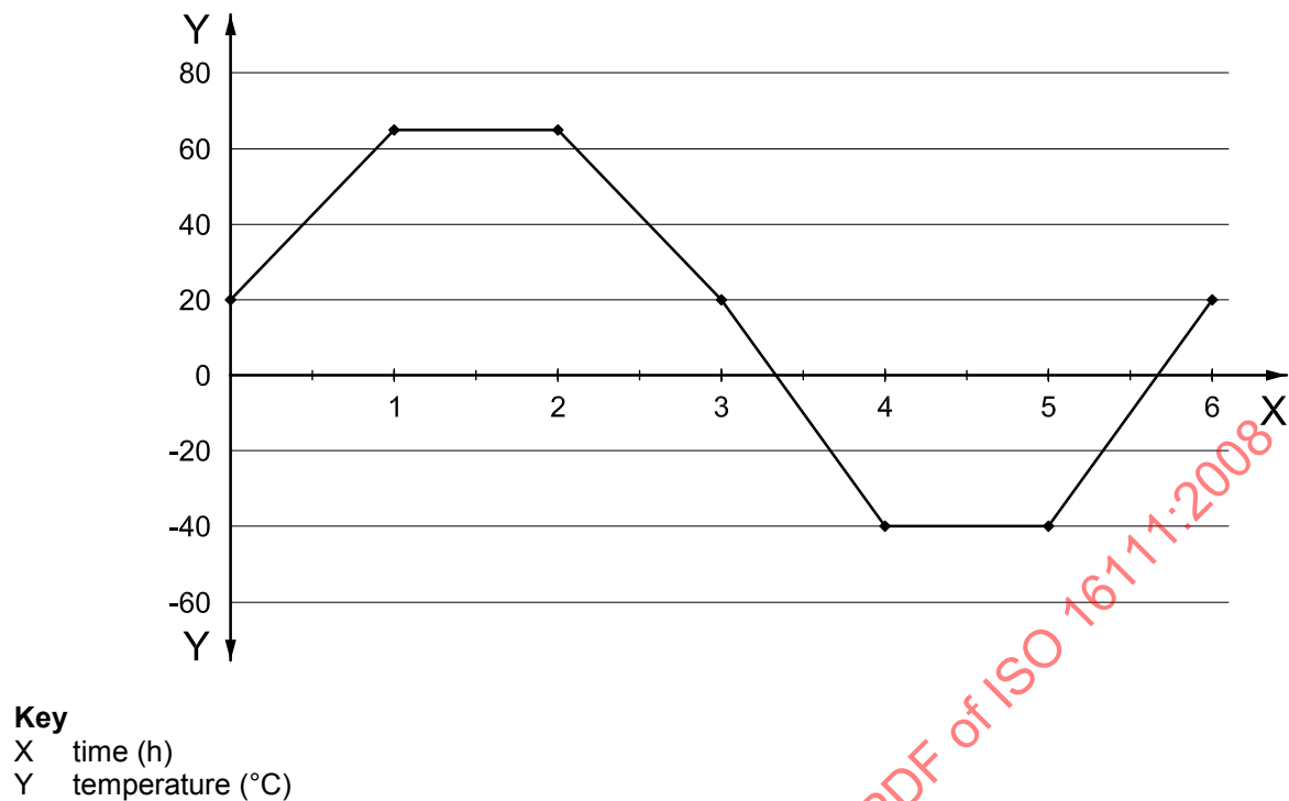
Figure 3 — Temperature cycling test example cycle
