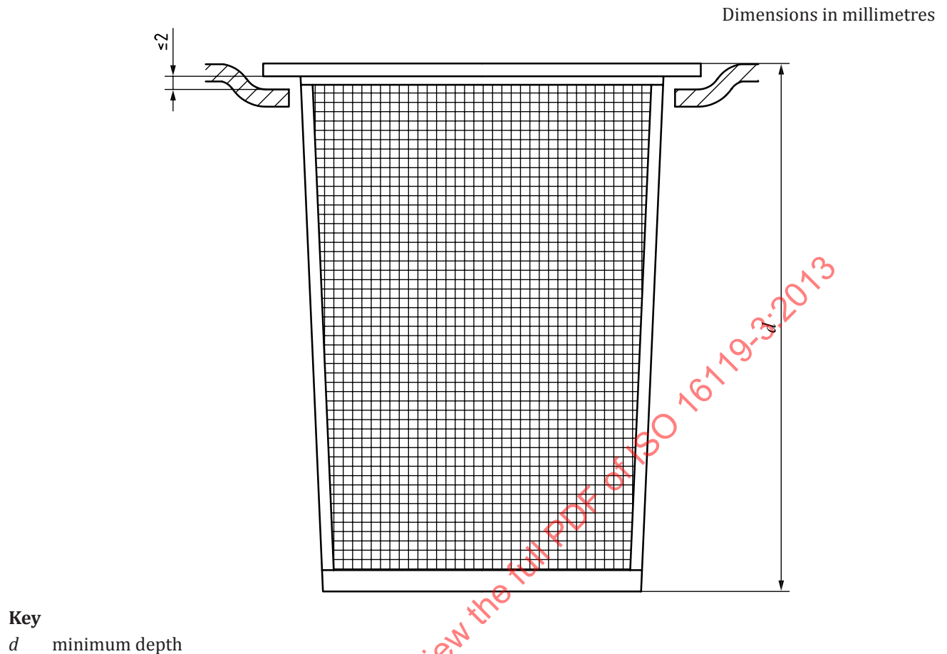
Figure 1 — Determination of the depth of the strainer and width of gap(s)
