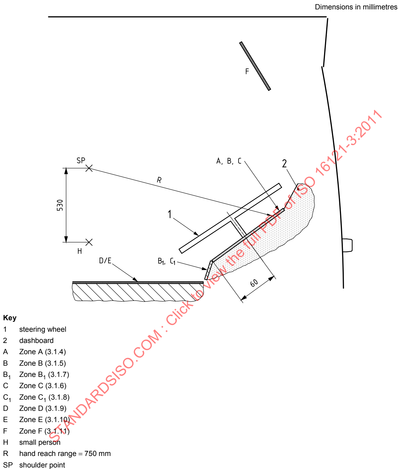
Figure 2 — Definitions of zones, side view
