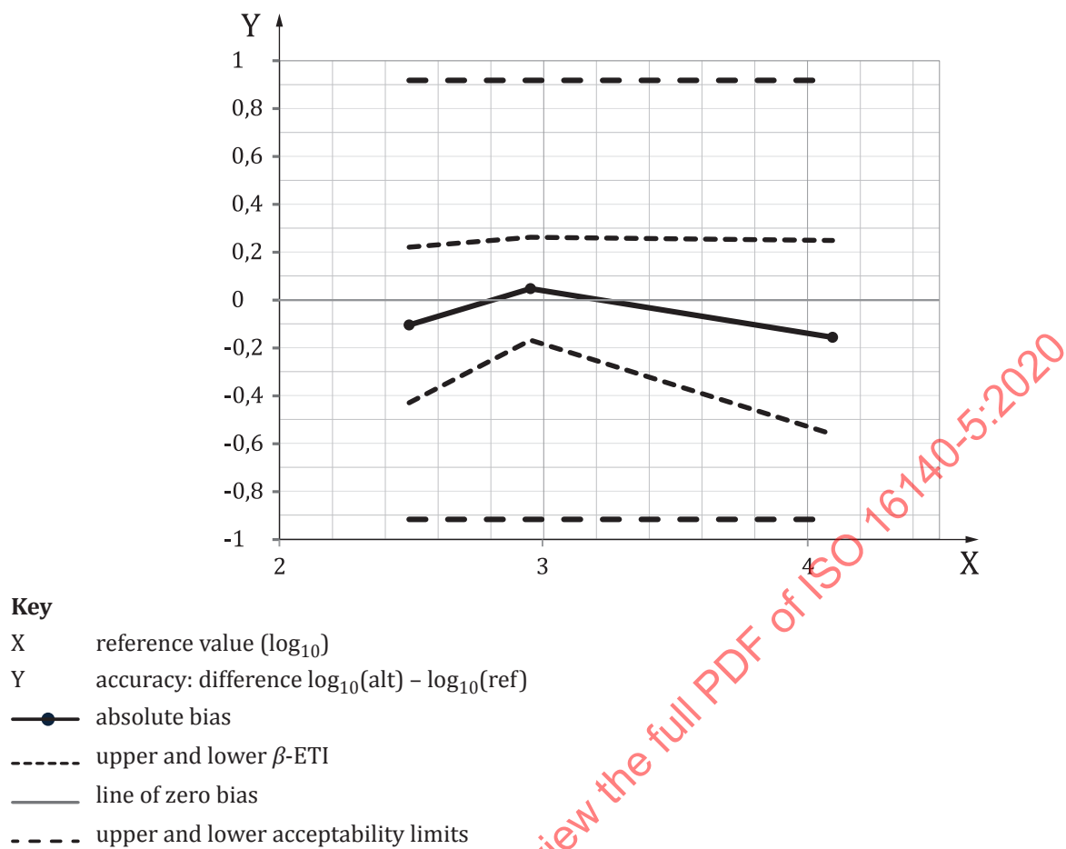
Figure B.4 — Accuracy profile of the alternative method using \beta = 80\% and corrected ALs based on the reproducibility standard deviation of the reference method in accordance with steps 8 and 9
