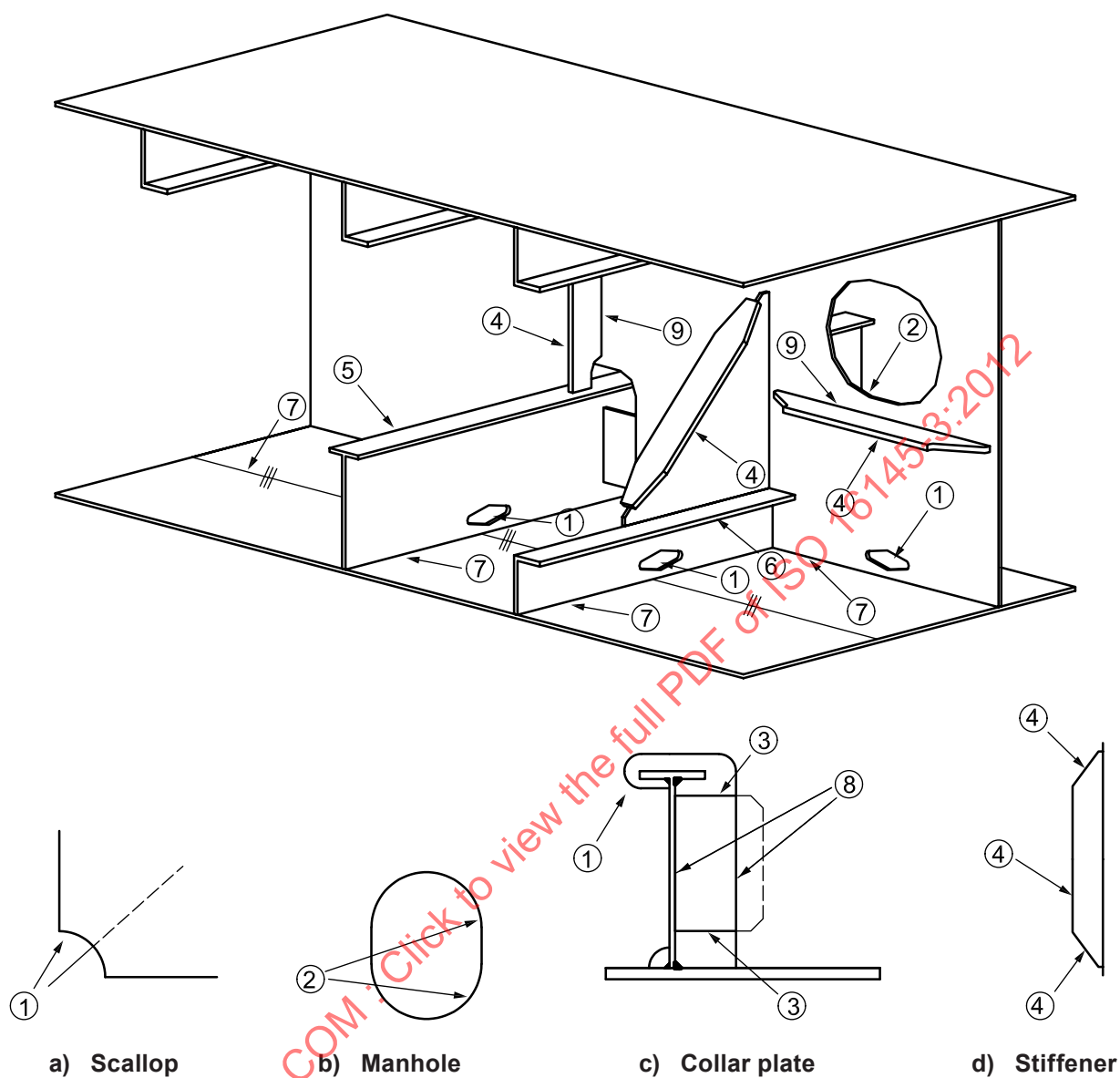
Figure 3 — Detail of stripe coating for each part
