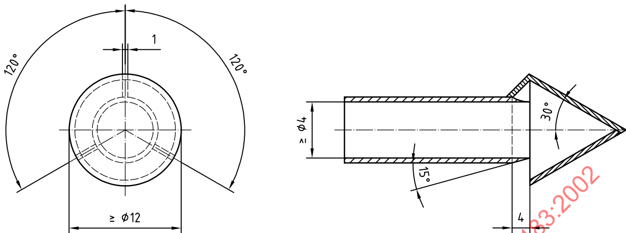
Figure 12 — Hatted probe
