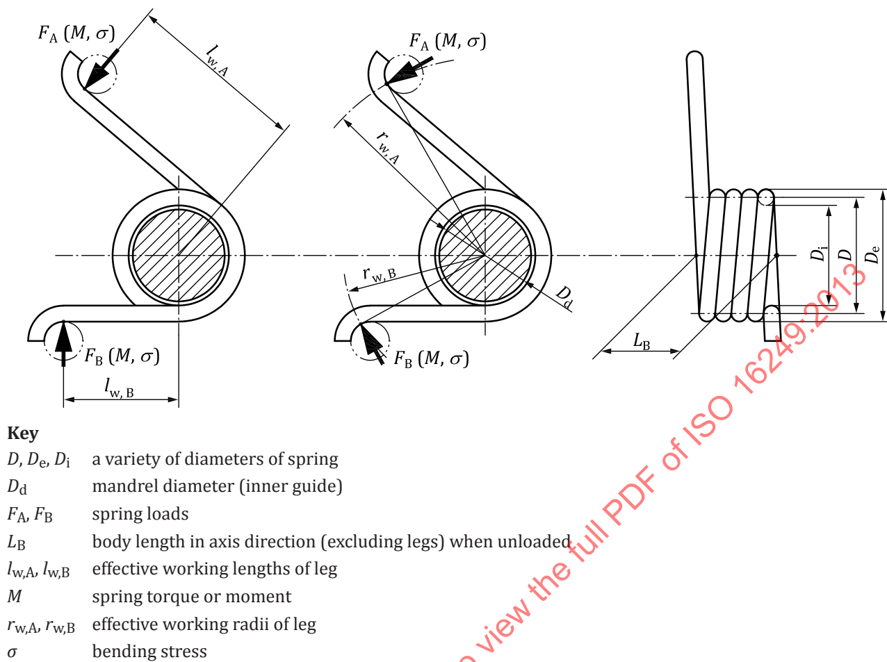
Figure 6 — Symbols for helical torsion spring related effective working length or radius of leg
