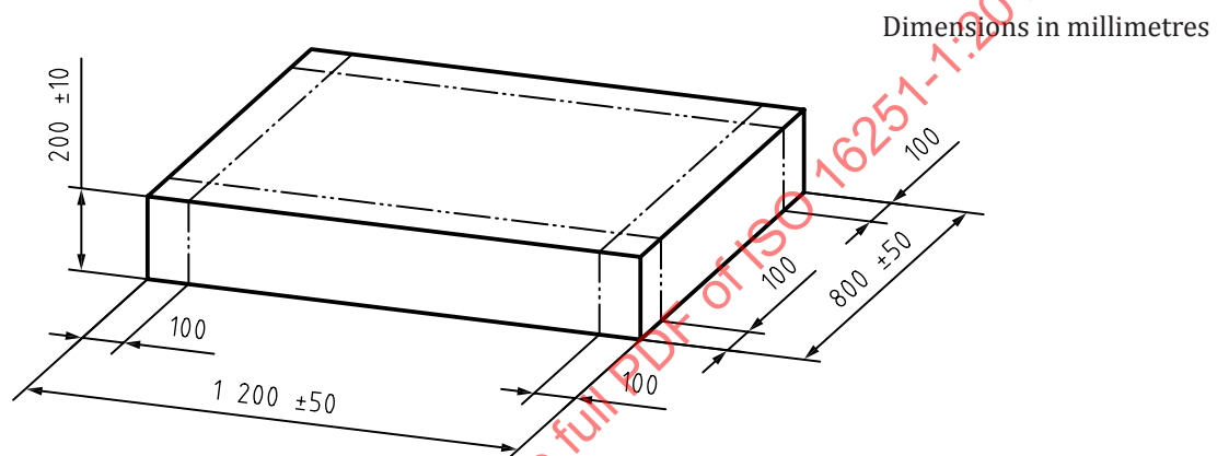
Figure A.1 — Concrete slab
