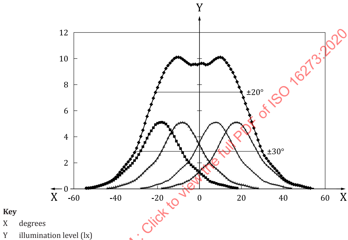
Figure B.1 — Horizontal angular power distribution of 4 IR illuminators and composite response
