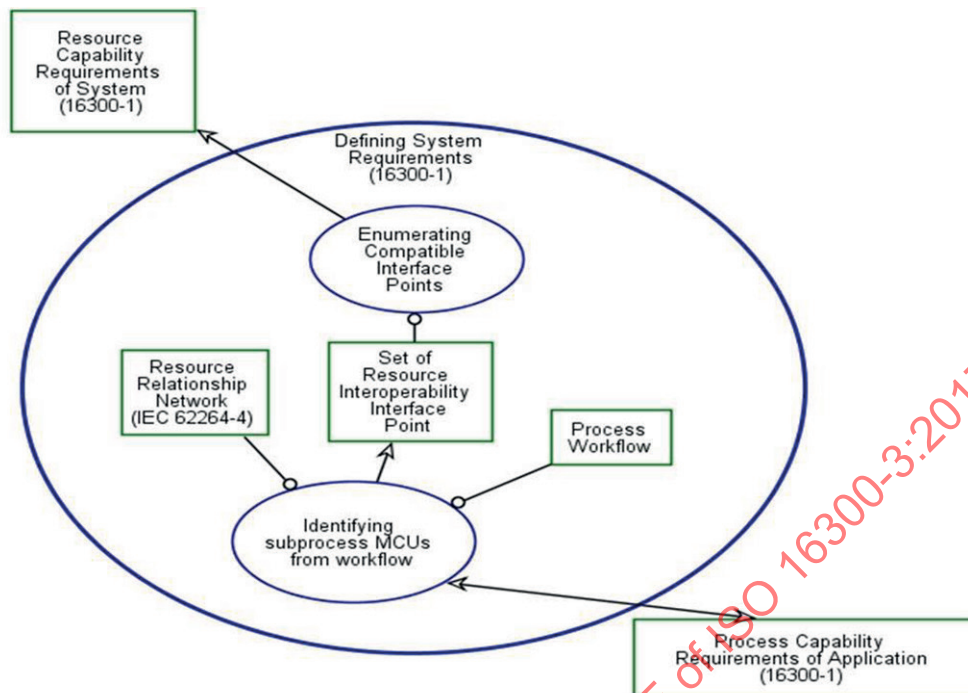
Figure 4 — Steps for interoperability requirements specification
