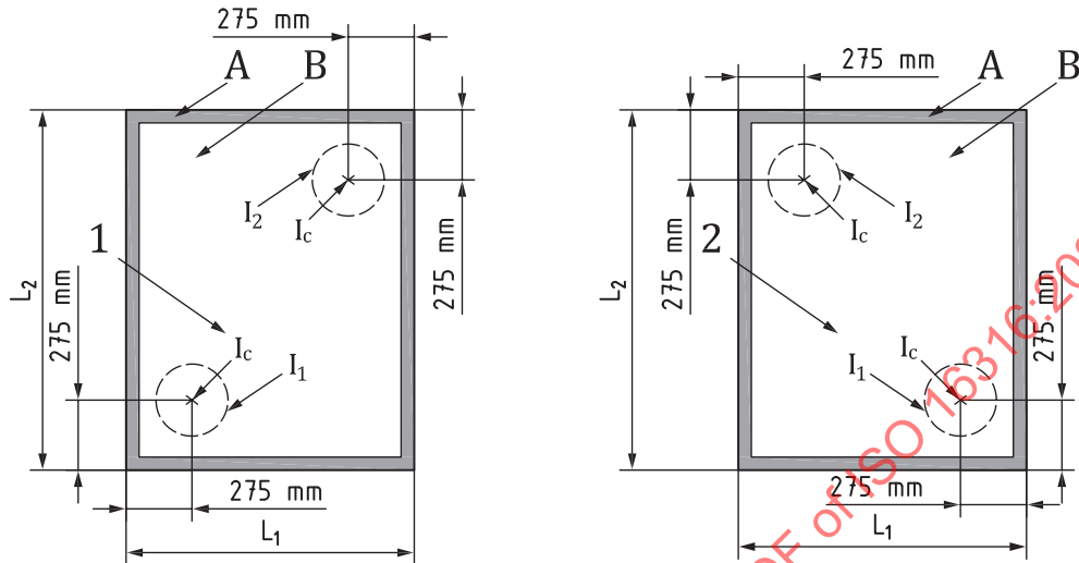
Figure E.3 — Default impact locations for substitutions based on a single specimen test
