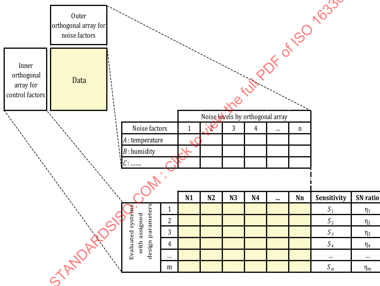
Figure 3 — Direct product plan for parameter design
