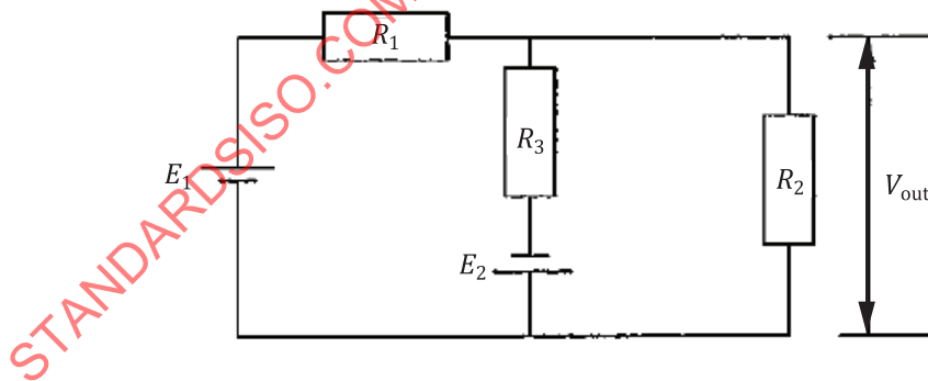
Figure 2 — Configuration of constant voltage circuit
