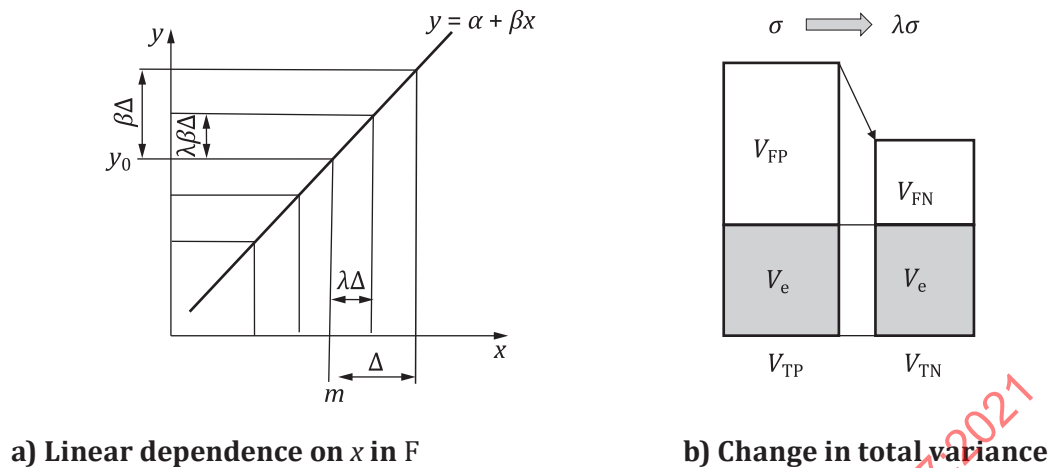
Figure 1 — Effect of changing \Delta in design parameter F on total variance
