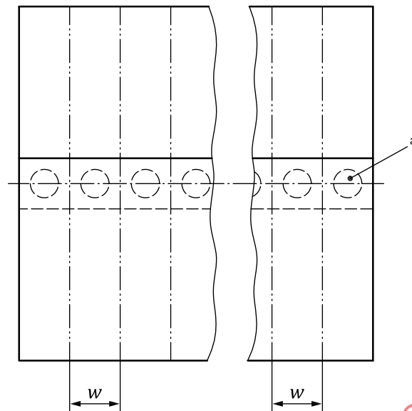
b) Multi weld spot test specimen
