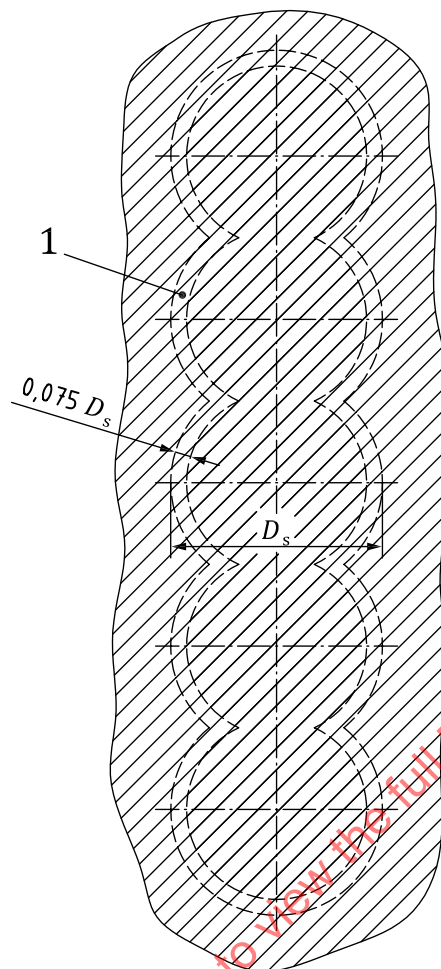
b) Nomenclature diagram of seam weld
