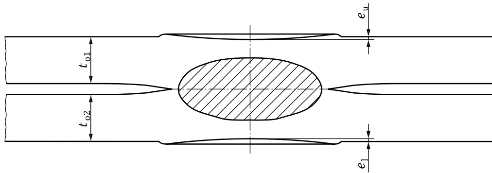
Figure 7 — Electrode indentation
