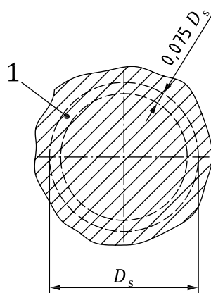
a) Nomenclature diagram of spot weld
