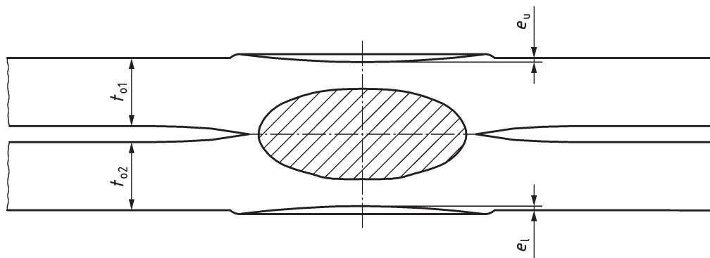
Figure 7 — Electrode indentation
