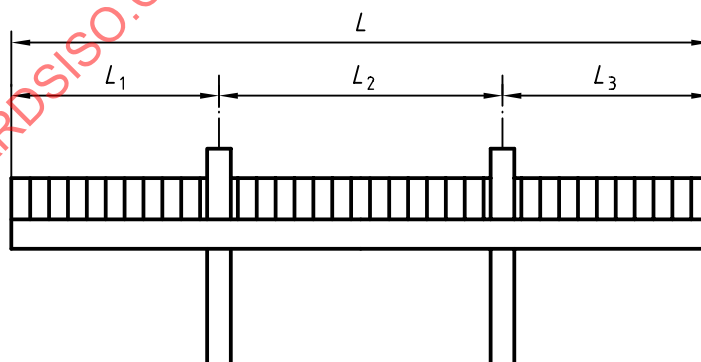
Figure 5 — Loading in the longitudinal direction for single-mast machines
