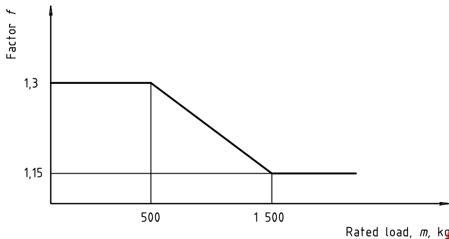
Figure 8 — Factor f as a function of rated load
