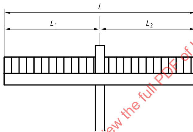
Figure 4 — Eccentric loading normal to the centreline
