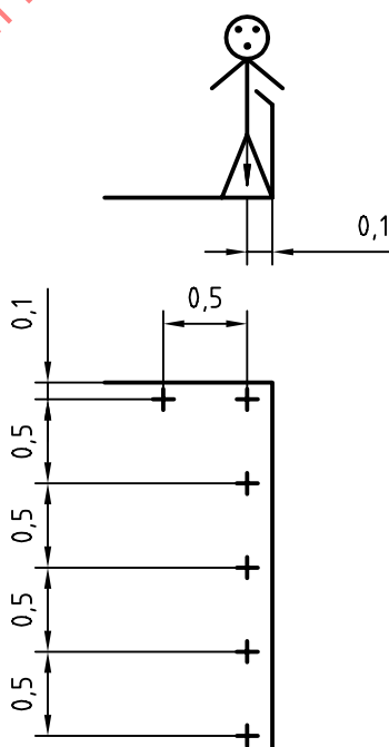
Figure 3 — Example of the distribution of persons on the main platform or platform extensions
