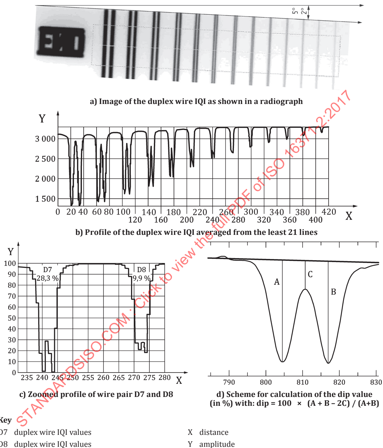
Figure A.1 — Example for duplex wire IQI evaluation with resulting IQI value D8
