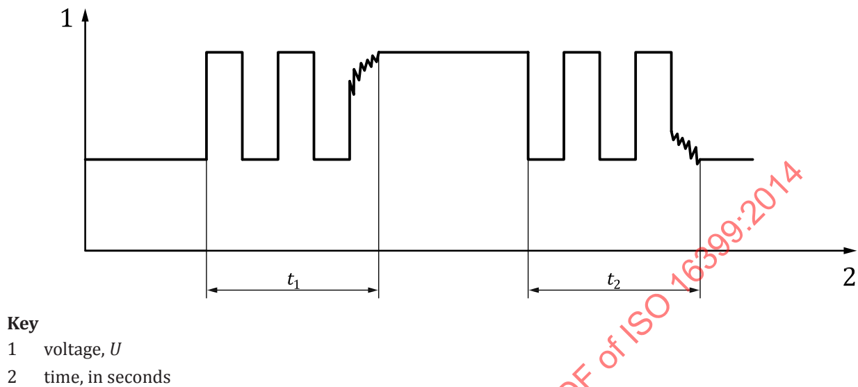
Figure A.4 — Bounce time
