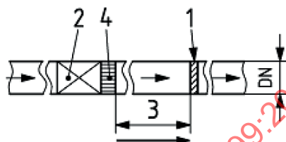
Test 2A: with a straightener
