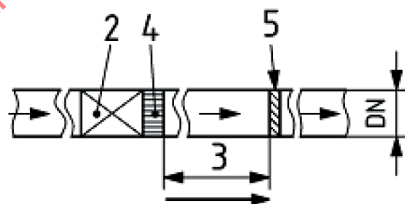
Test 4A: with a straightener
