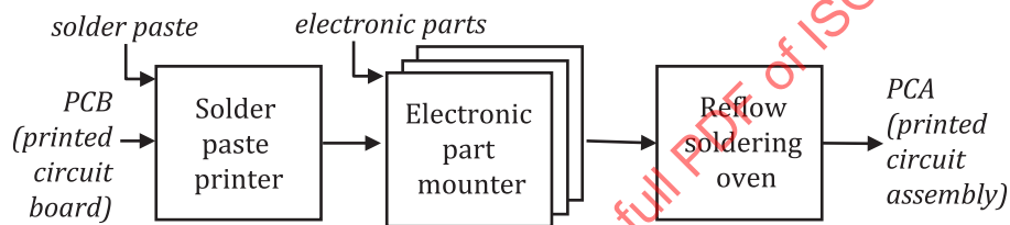
Figure B.1 — Structure of printed circuit assembly (PCA) line
