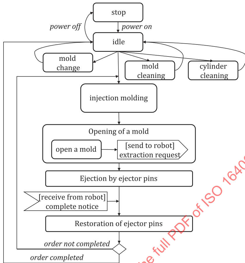
Figure C.2 — Activity diagram for an injection molding machine
