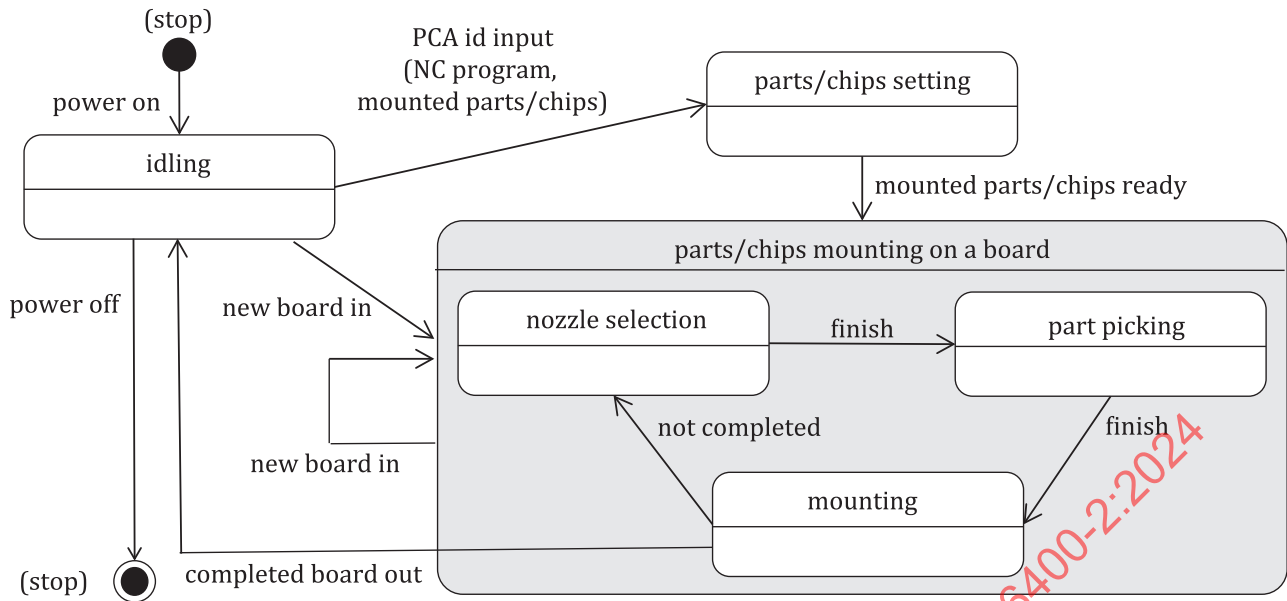
Figure B.3 — Activity diagram for an electronic part mounter
