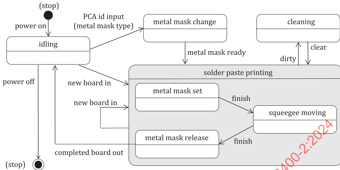
Figure B.2 — Activity diagram for a solder paste printer
