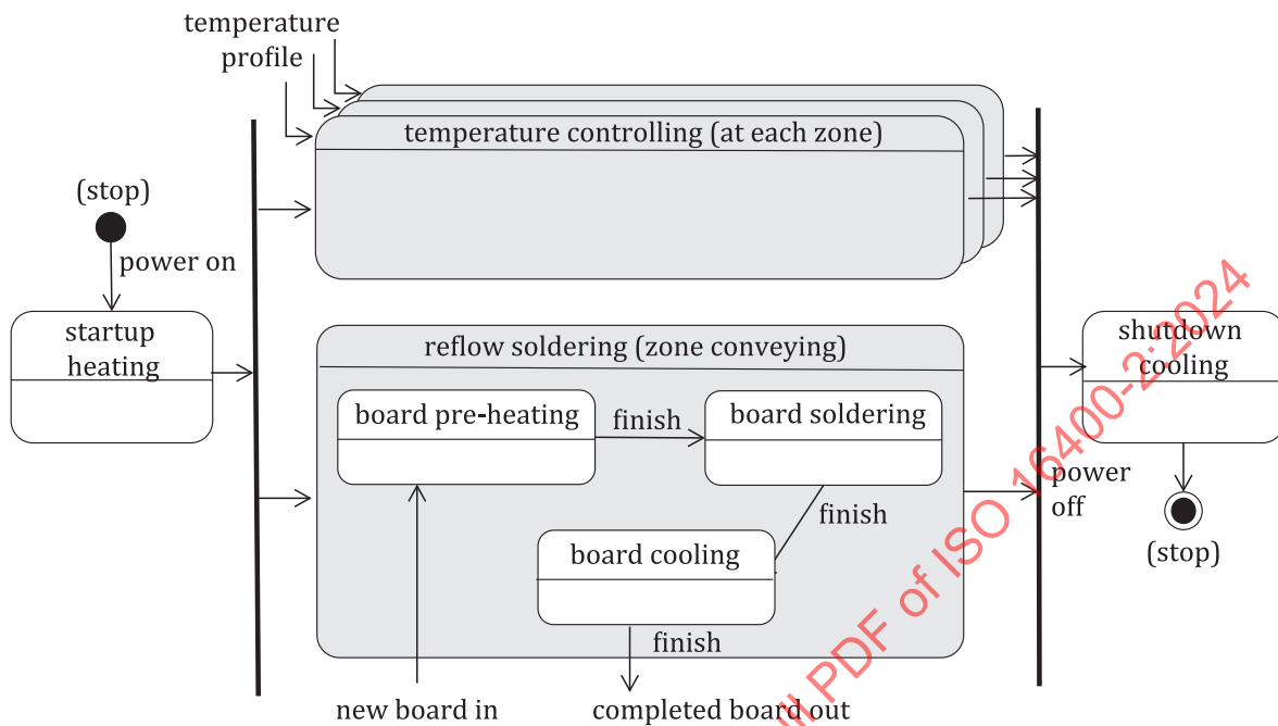
Figure B.4 — Activity diagram for a reflow soldering oven
