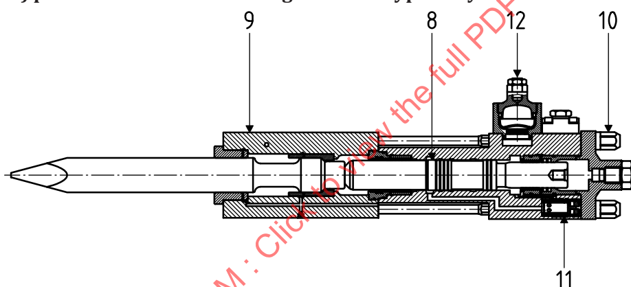
b) power cell for oil and nitrogen driven type of hydraulic breakers
