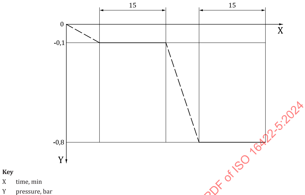
Figure 2 — Negative-pressure test regime
