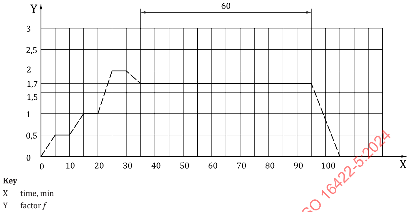
Figure 1 — Hydrostatic pressure test regime
