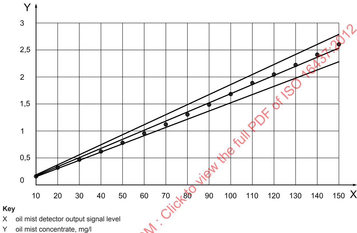
Figure A.2 — Sample of calibration result of oil mist detector output signal
